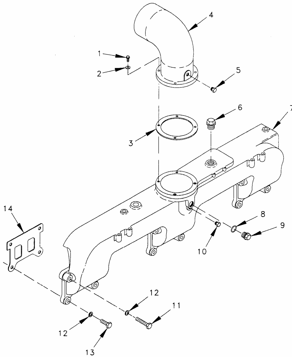
Figure 34. Intake Manifold Group.
