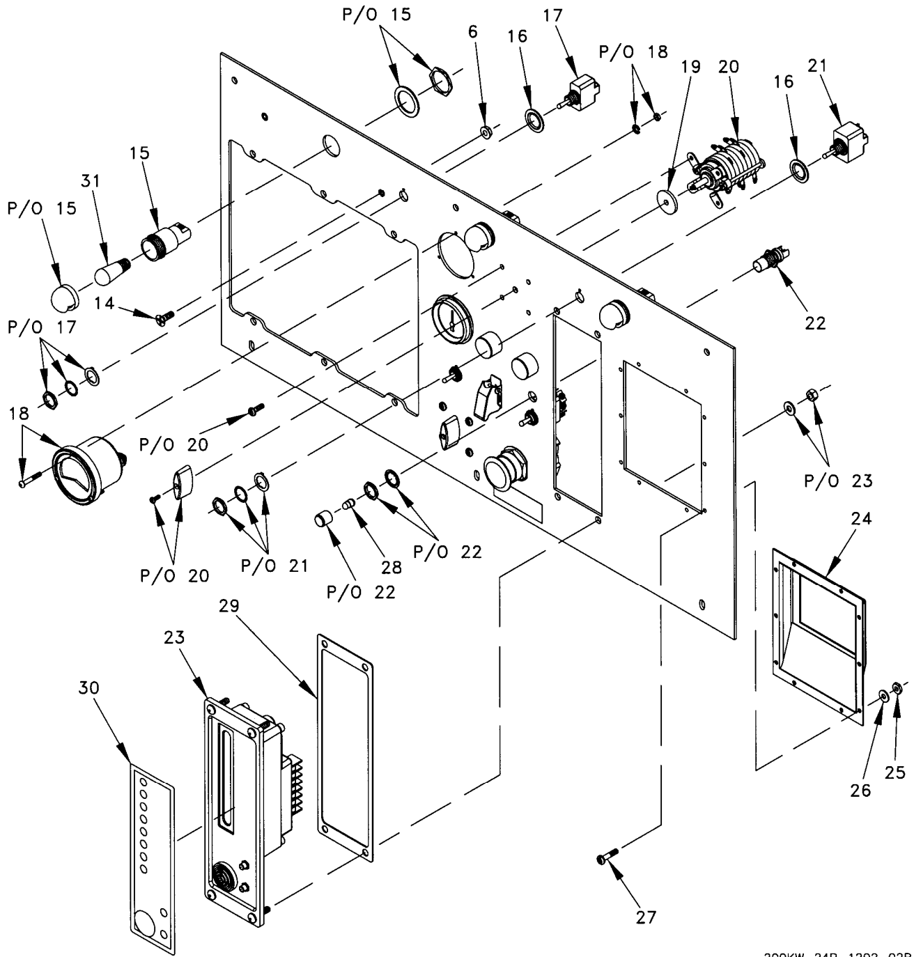
Figure 6. Control Box Panel Assembly (Sheet 2 of 3).
