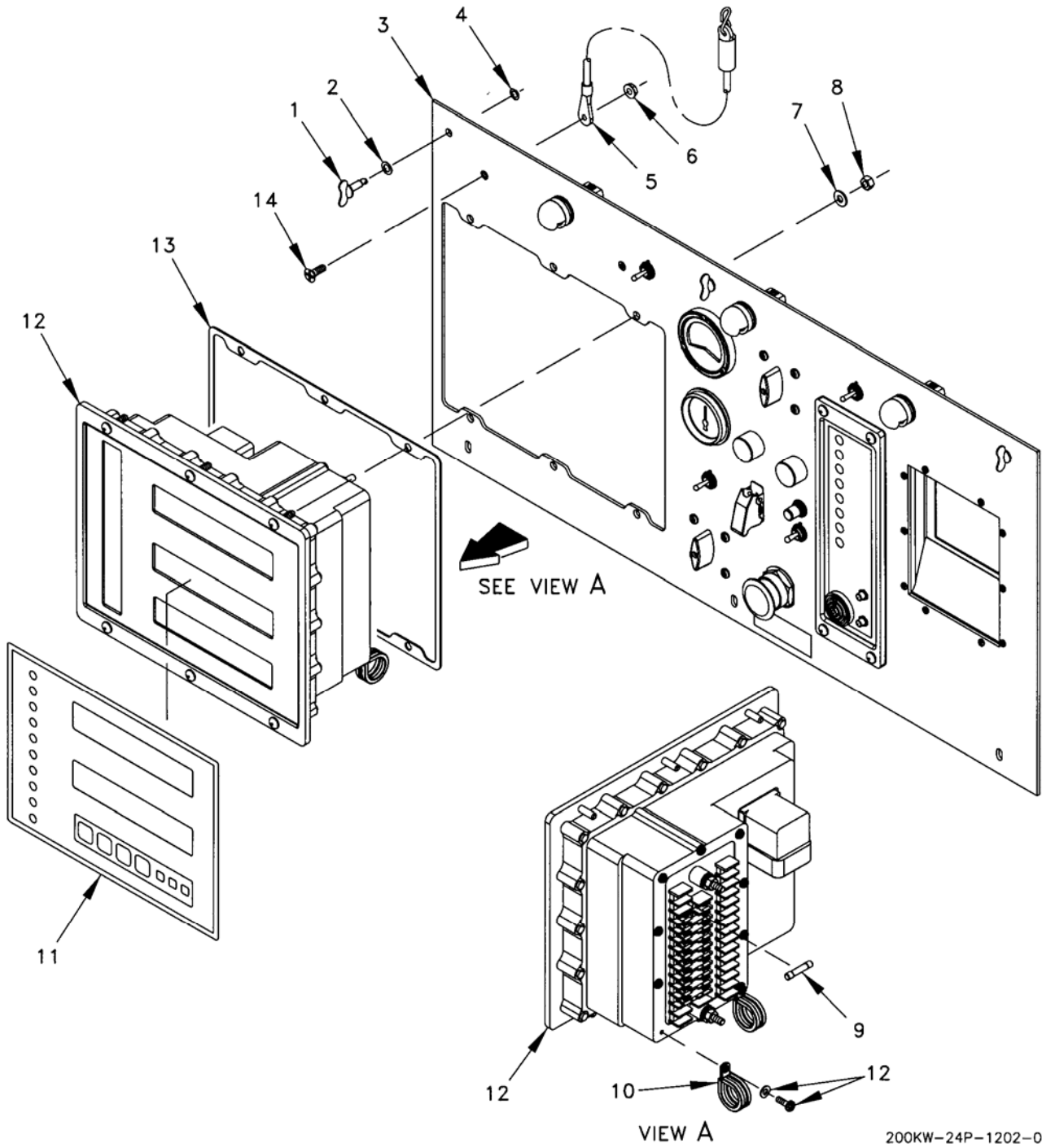
Figure 6. Control Box Panel Assembly (Sheet 1 of 3).
