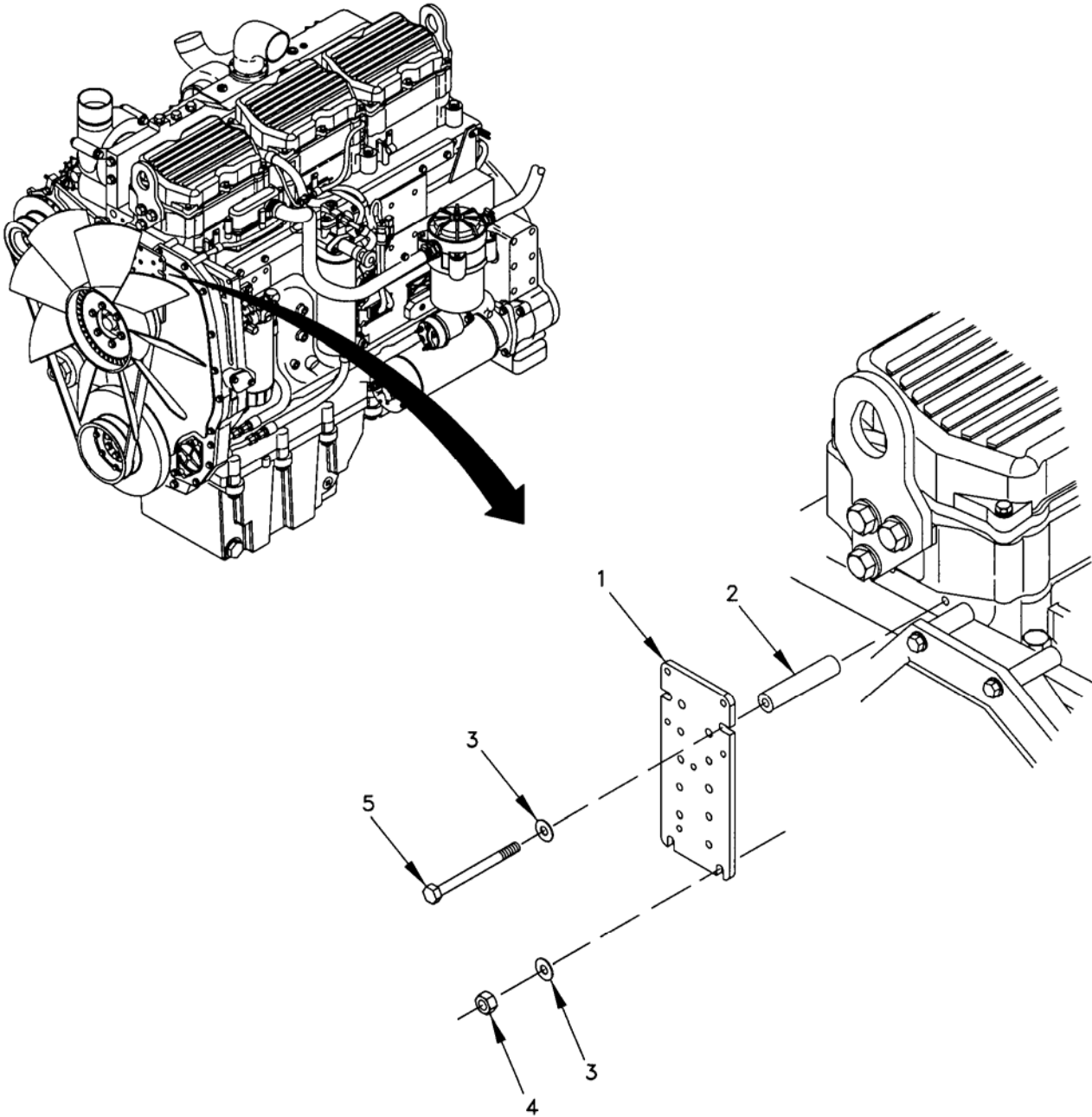
Figure 21. Fan Drive Mounting Group.
