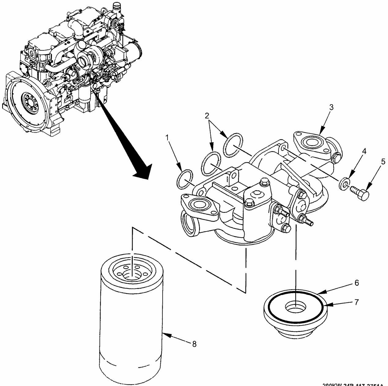
Figure 37. Oil Filter Group.
