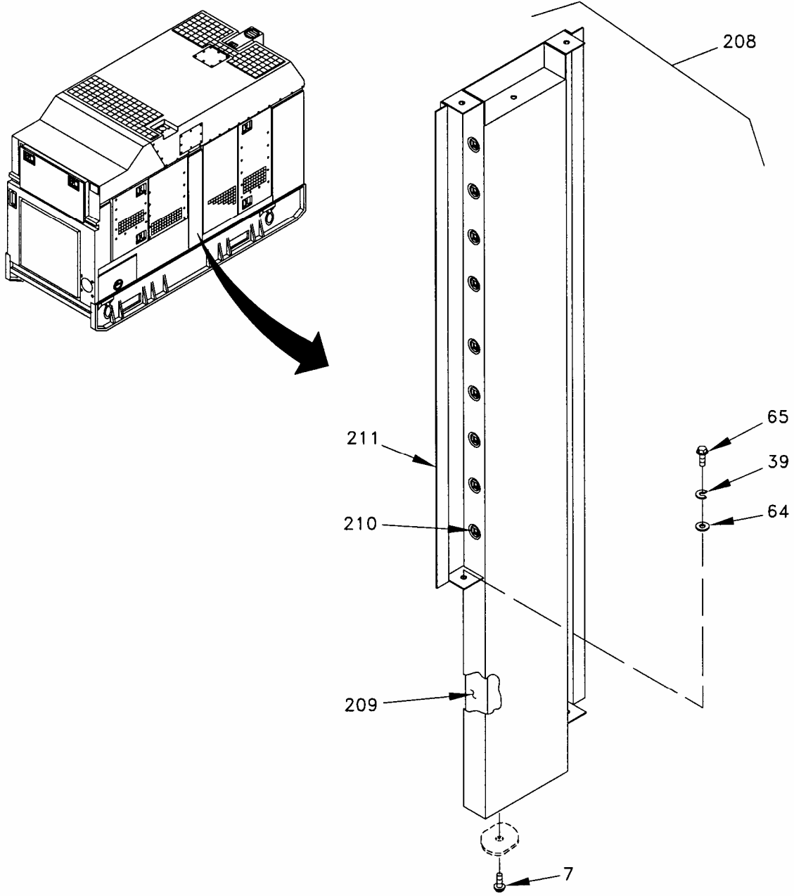
Figure 3. Housing Installation (Sheet 17 of 27).
