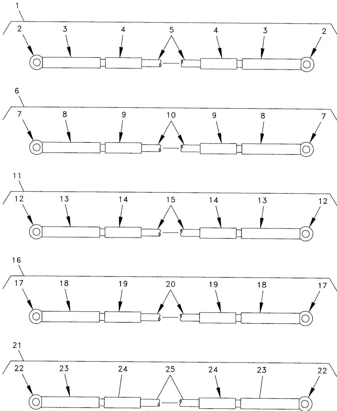
Figure 8. Cable Assemblies (Sheet 1 of 5).
