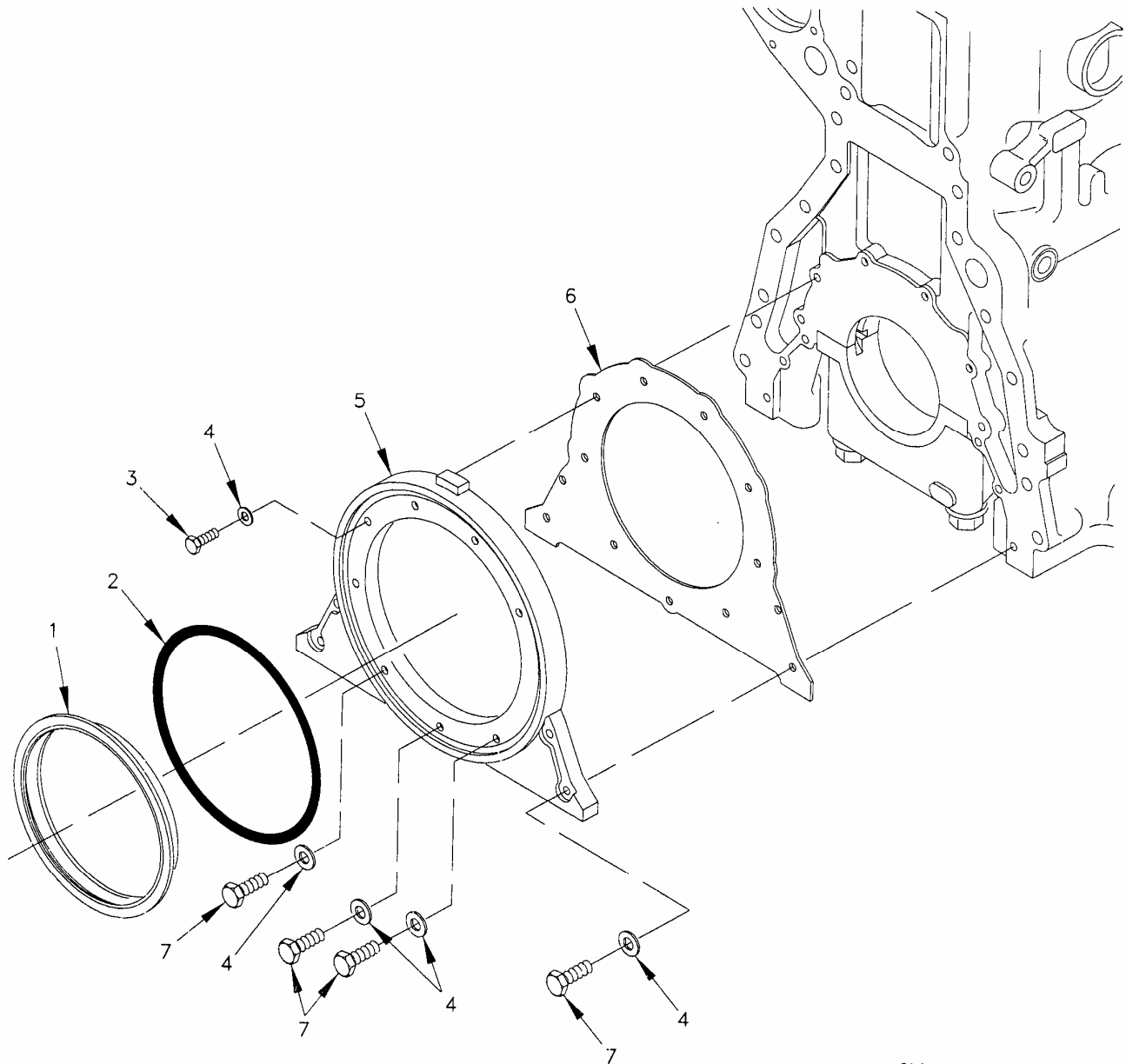
Figure 53. Crankshaft Seal Group.
