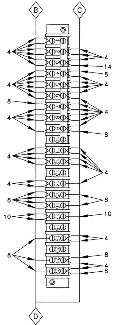
Figure 5. Control Box Harness Assembly (Sheet 2 of 5).
