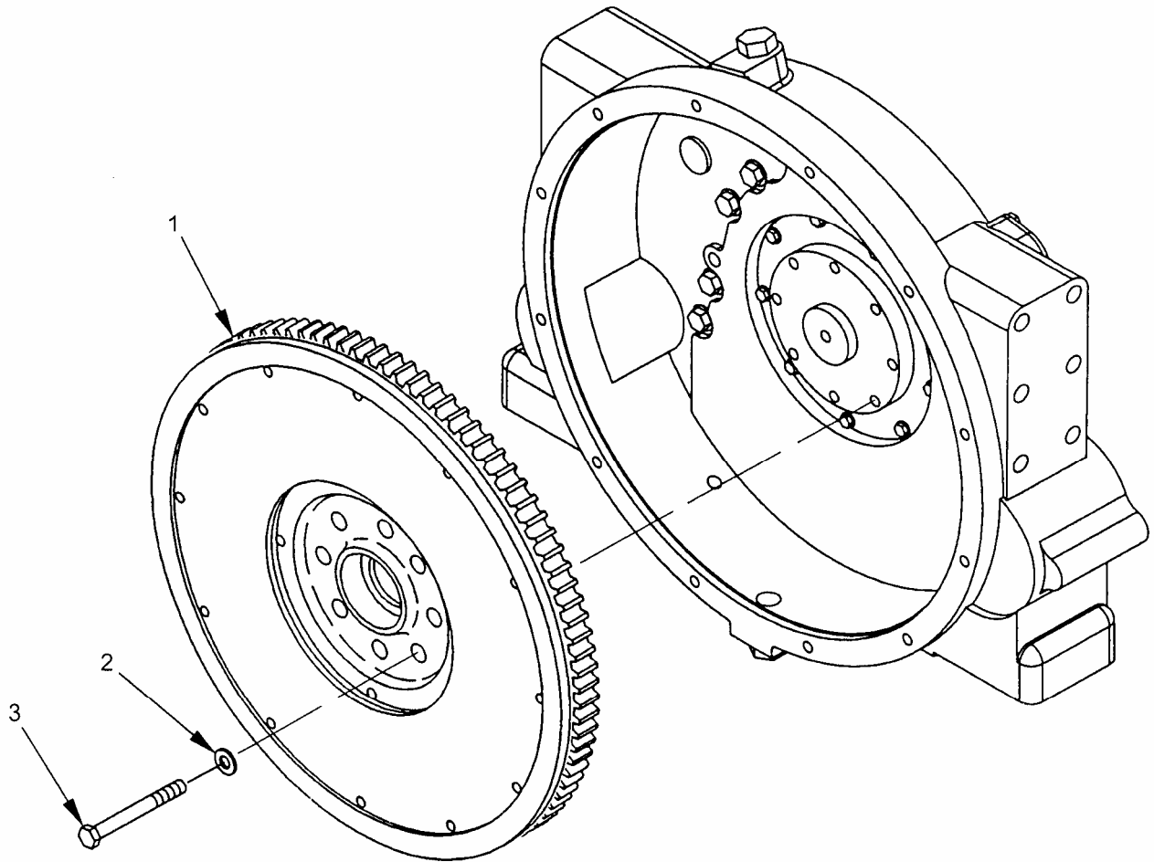
Figure 49. Flywheel Group.
