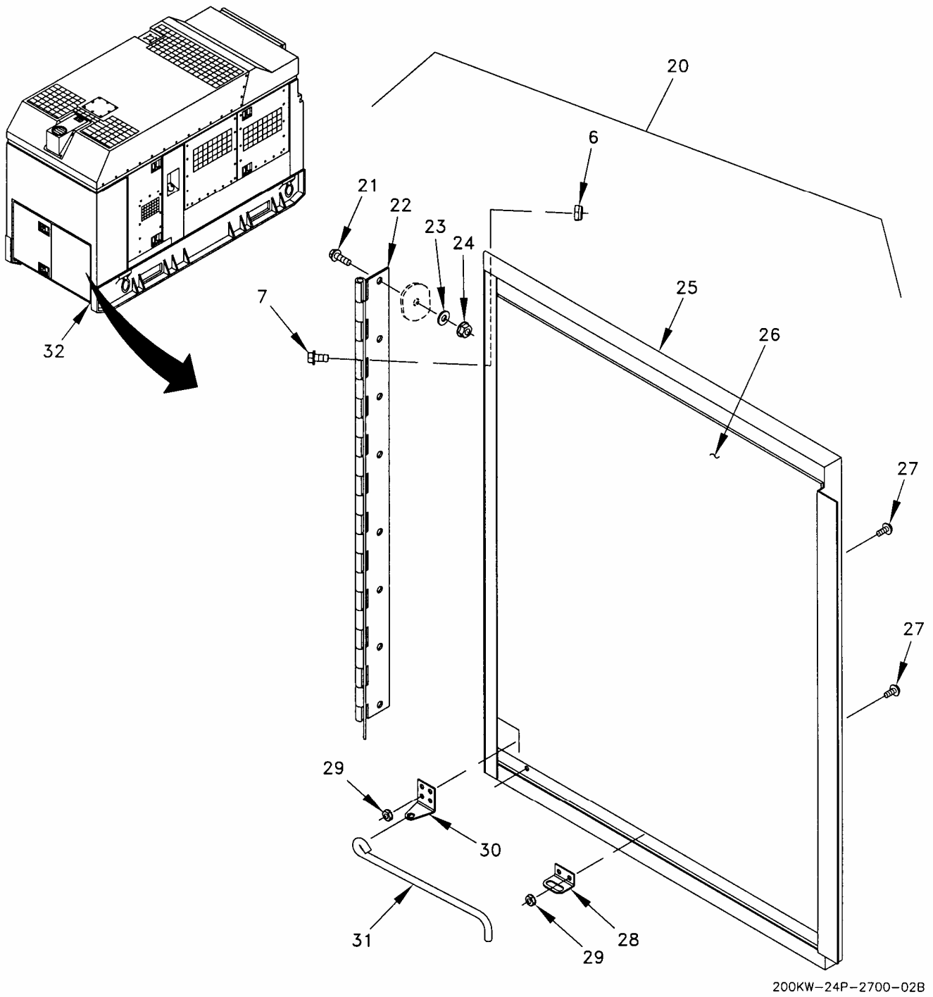
Figure 3. Housing Installation (Sheet 2 of 27).
