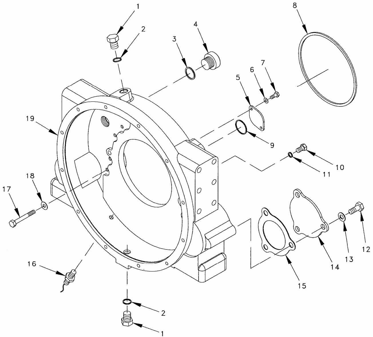
Figure 50. Flywheel Housing Group.
