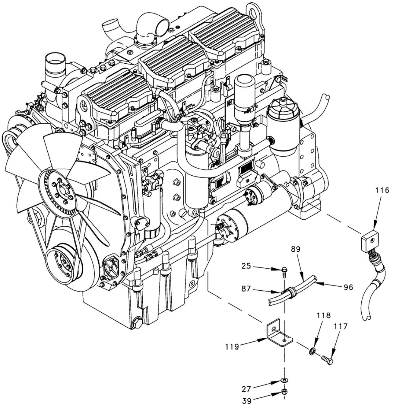
Figure 7. Electrical Components Installation (Sheet 9 of 9).
