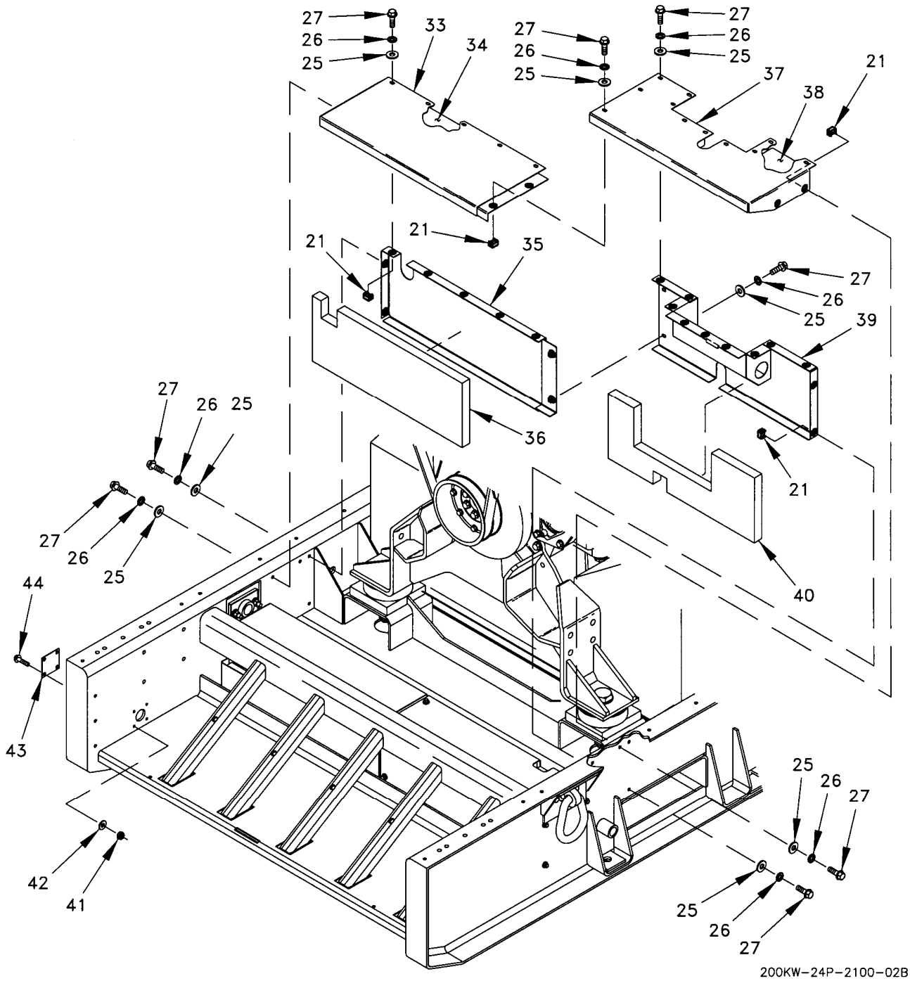
Figure 16. Engine Generator Base Assembly (Sheet 2 of 4).
