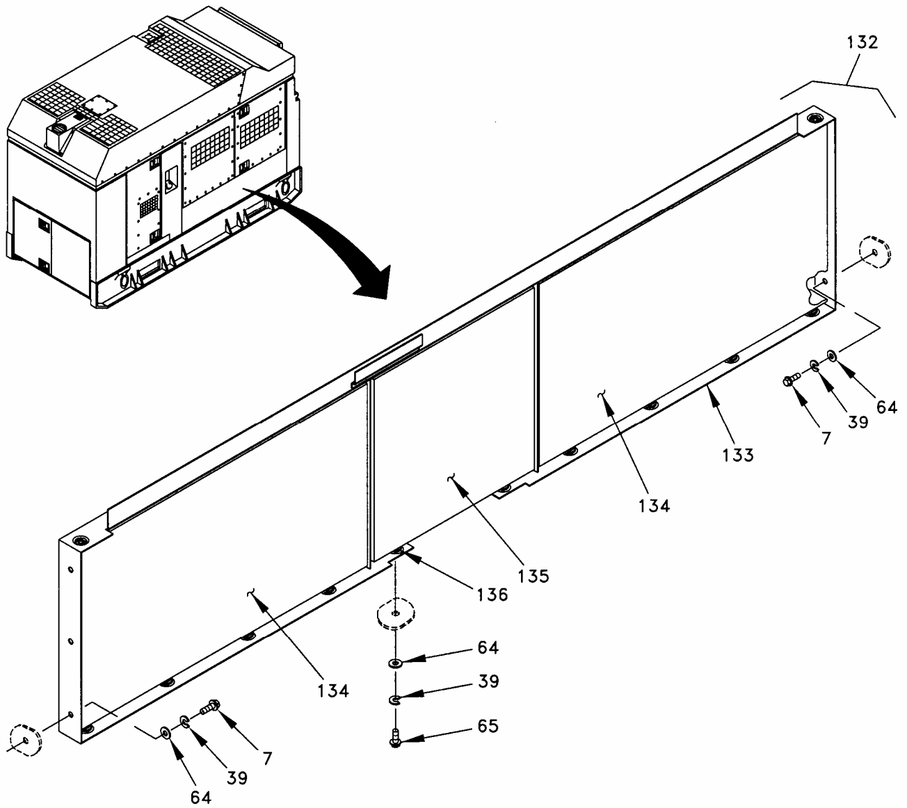
Figure 3. Housing Installation (Sheet 9 of 27).
