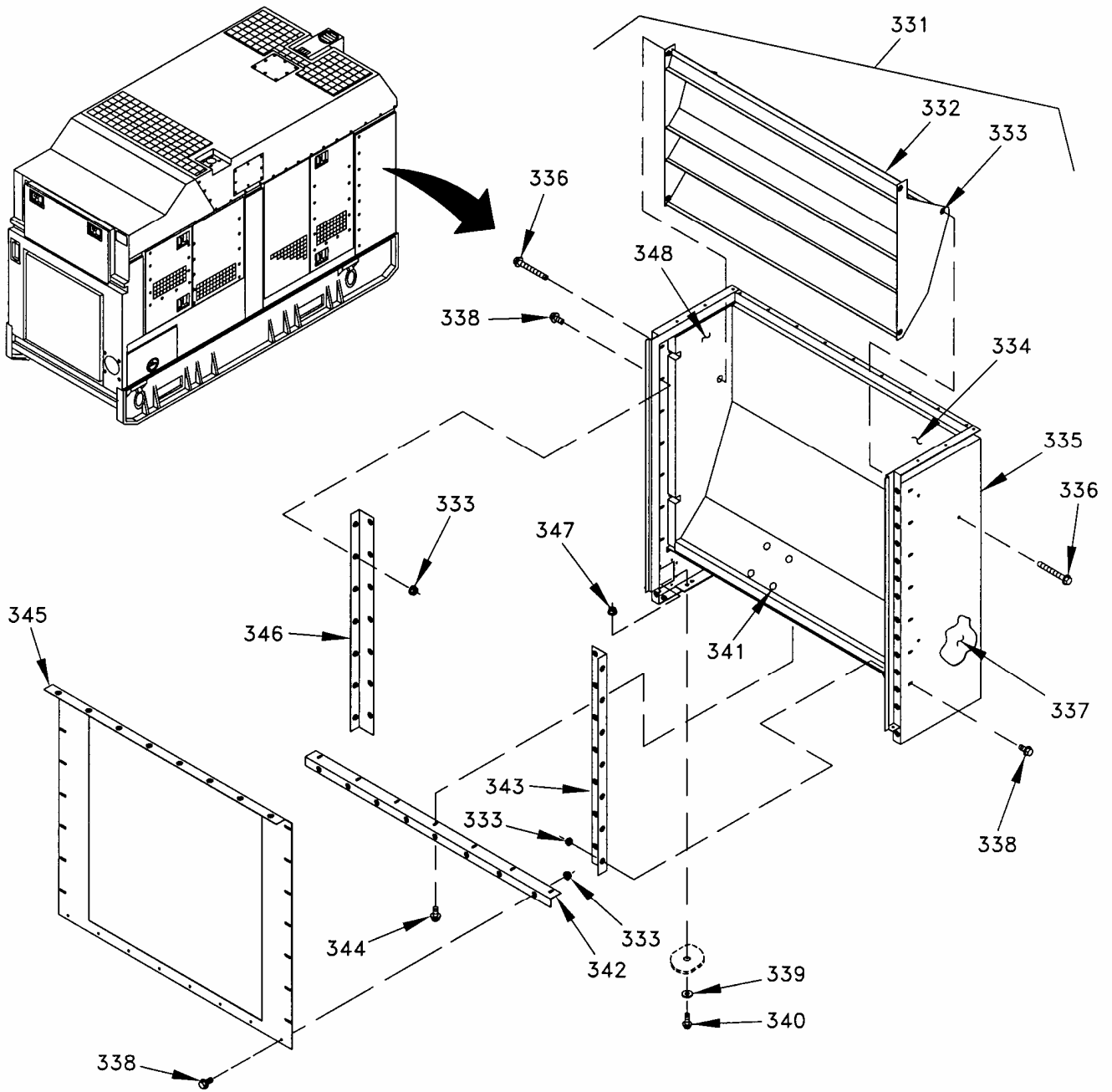
Figure 3. Housing Installation (Sheet 26 of 27).
