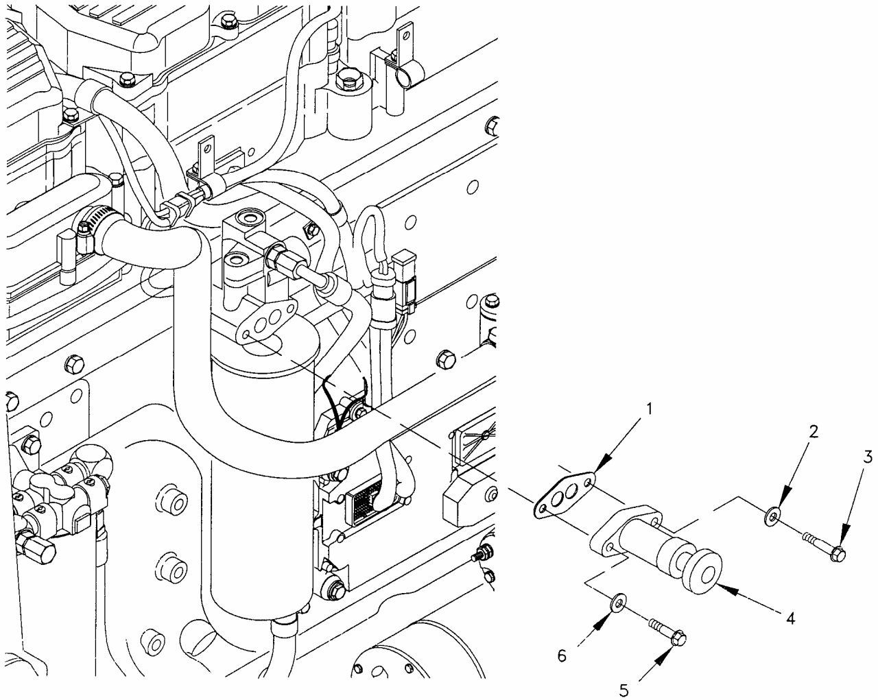
Figure 42. Priming Fuel Pump Group.
