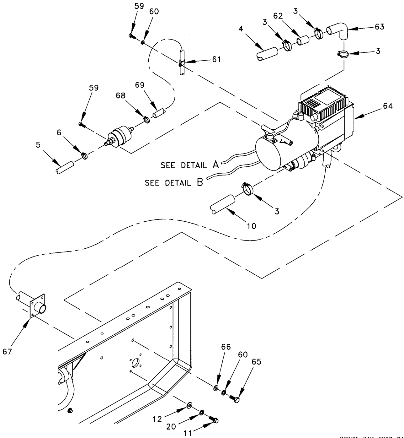
Figure 60. Winterization Group (Sheet 4 of 5).
