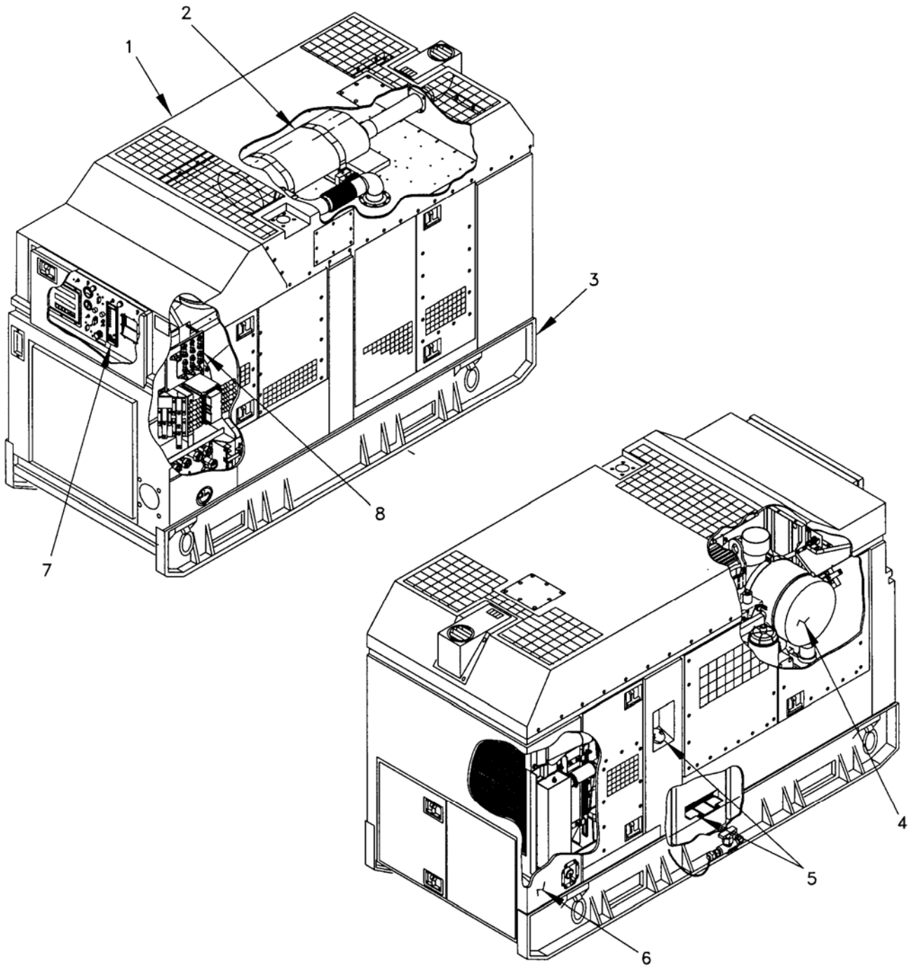
Figure 2. Generator Set Assembly.
