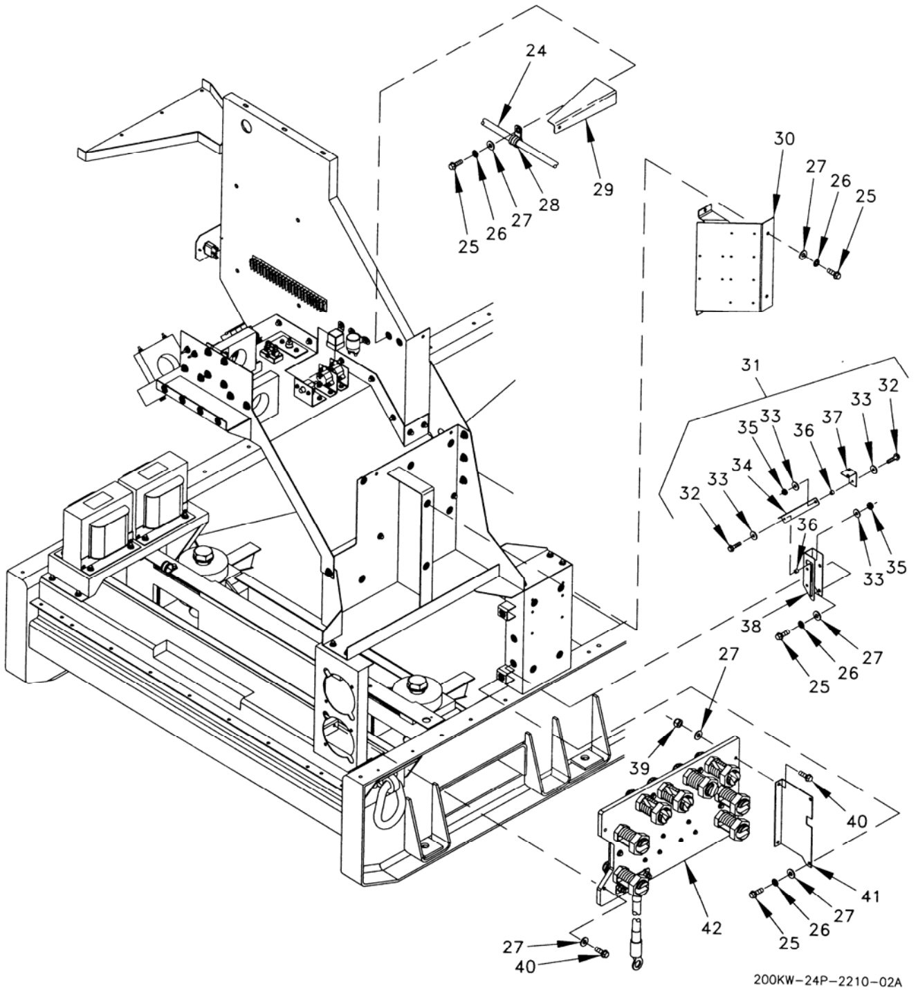
Figure 7. Electrical Components Installation (Sheet 2 of 9).
