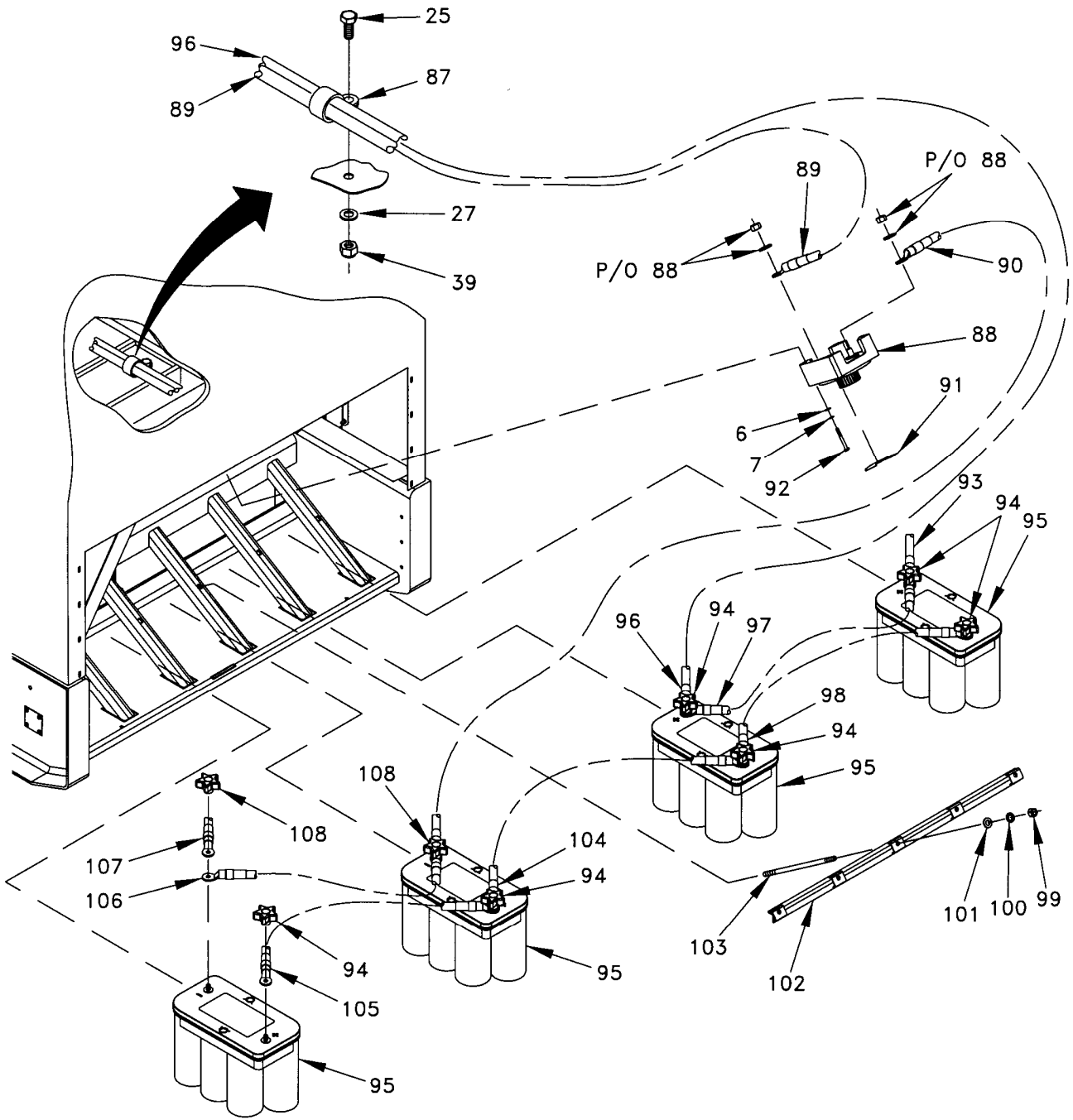
Figure 7. Electrical Components Installation (Sheet 7 of 9).
