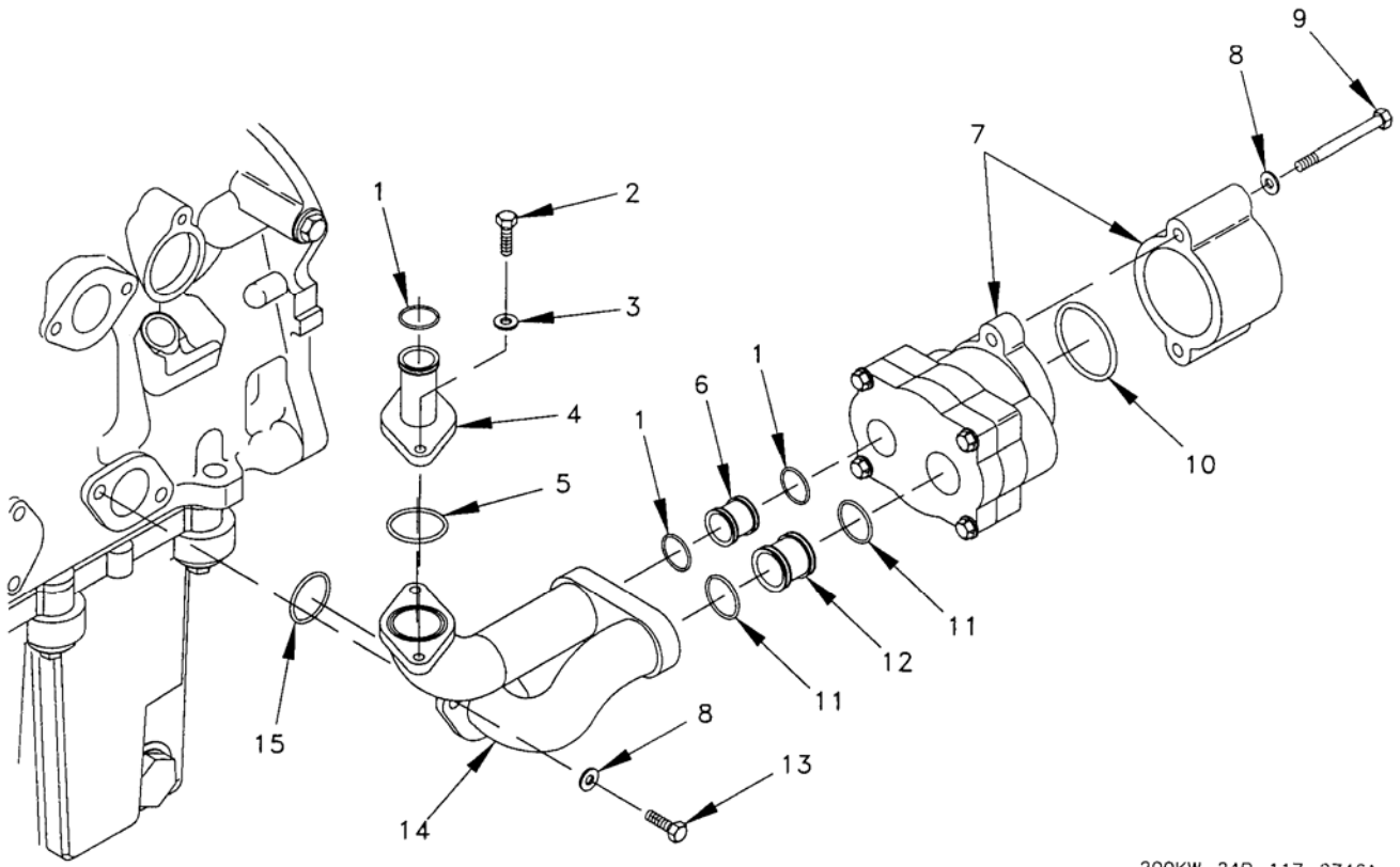
Figure 36. Oil Pump Group.
