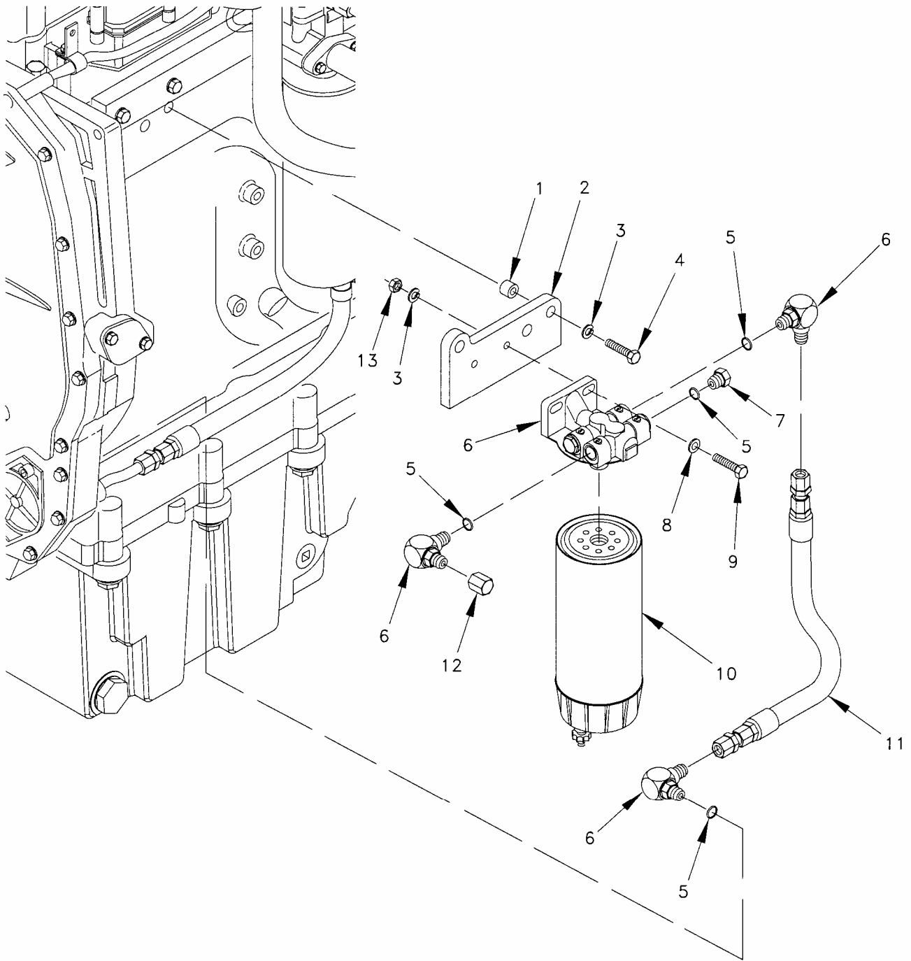
Figure 44. Primary Fuel Group.
