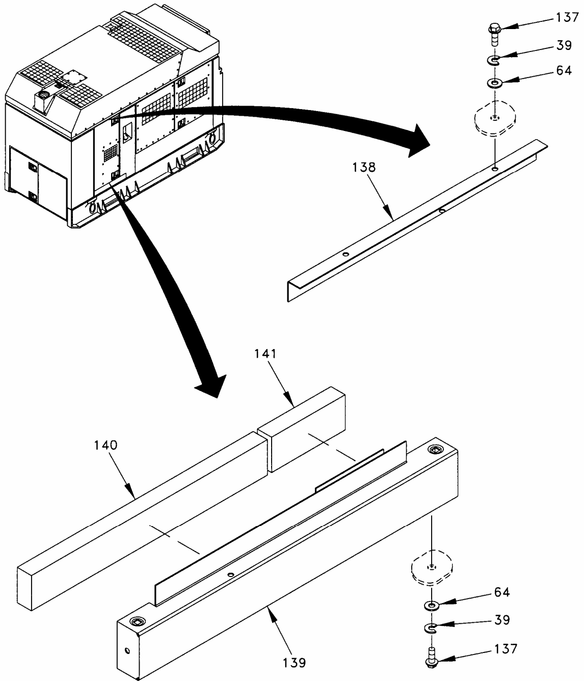
Figure 3. Housing Installation (Sheet 10 of 27).
