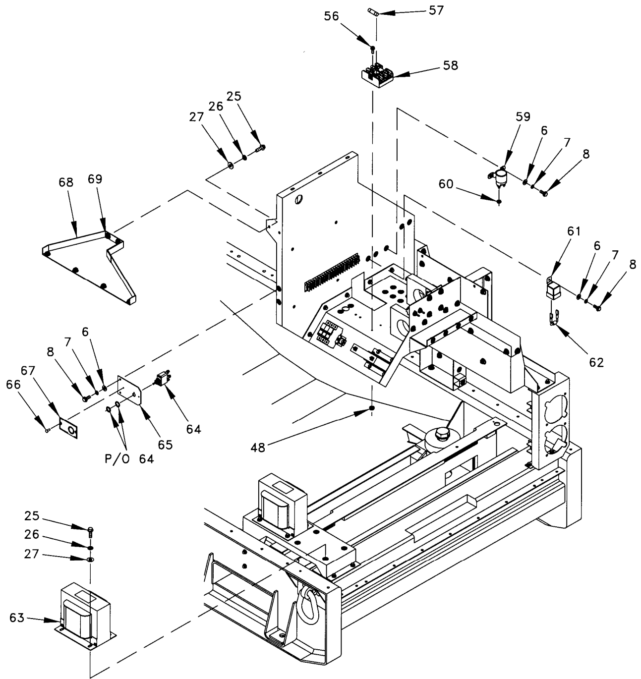
Figure 7. Electrical Components Installation (Sheet 4 of 9).
