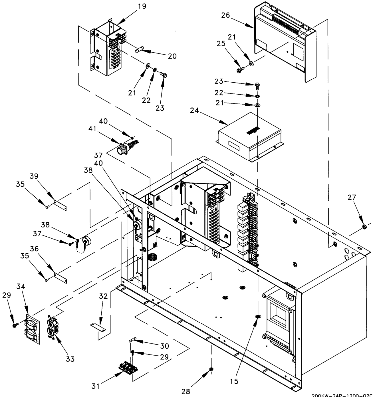
Figure 4. Control Box Assembly (Sheet 2 of 5).
