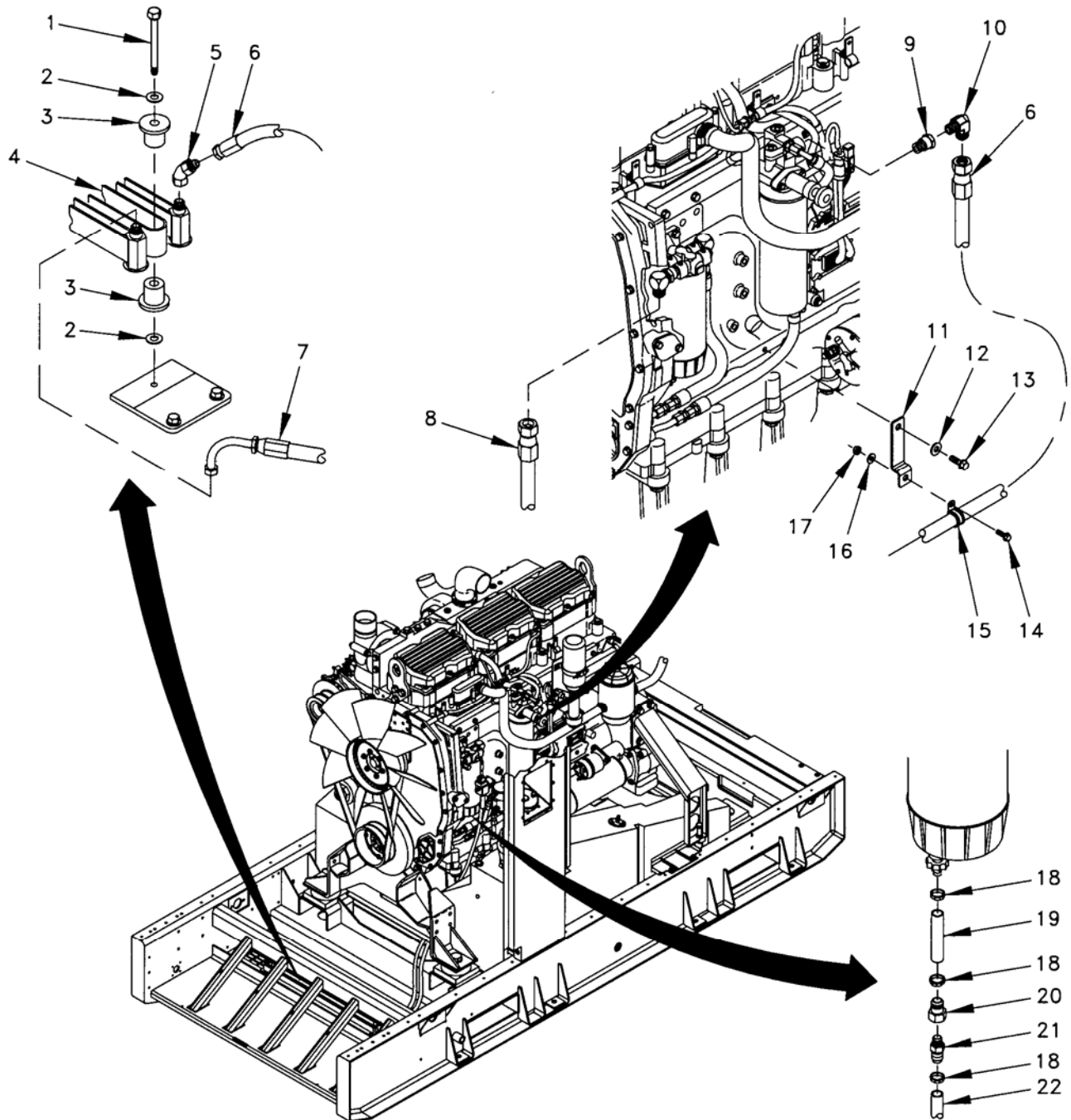
Figure 12. Fuel System Installation (Sheet 1 of 4).
