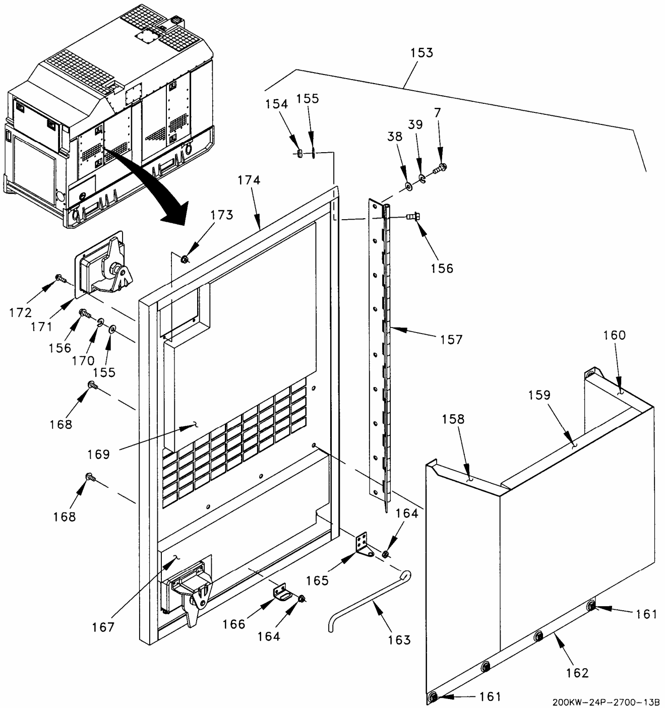
Figure 3. Housing Installation (Sheet 13 of 27).
