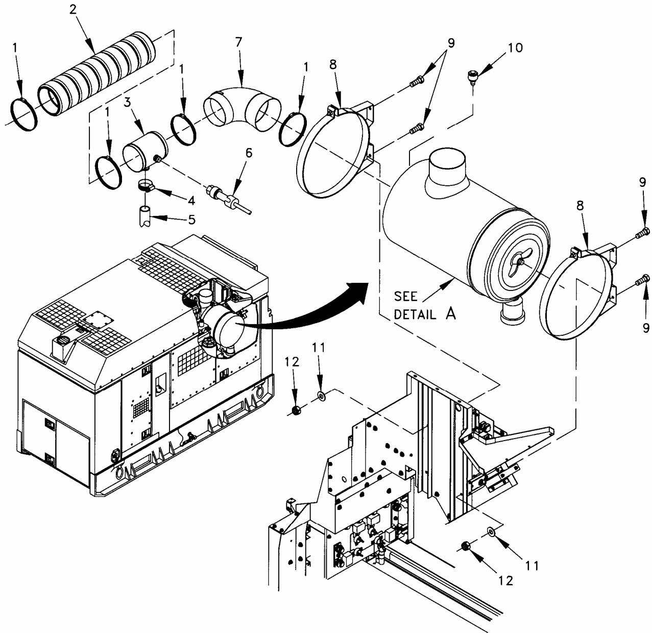
Figure 15. Air Cleaner Installation (Sheet 1 of 3).
