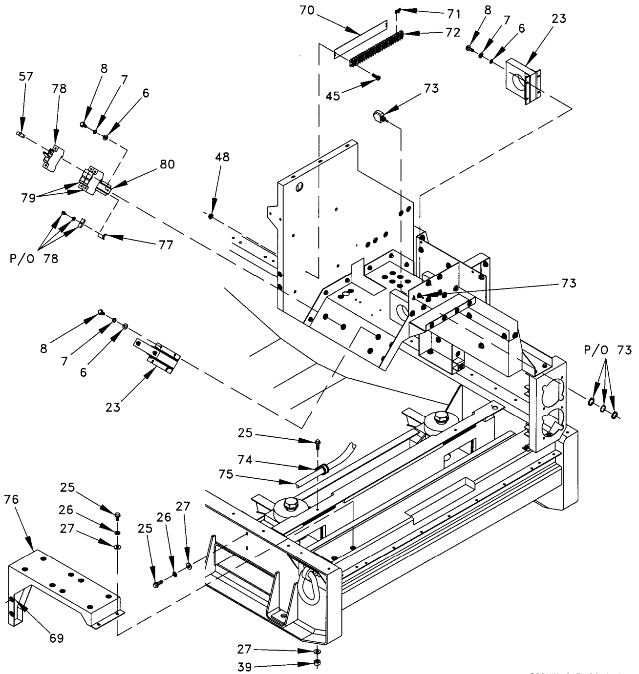
Figure 7. Electrical Components Installation (Sheet 5 of 9).
