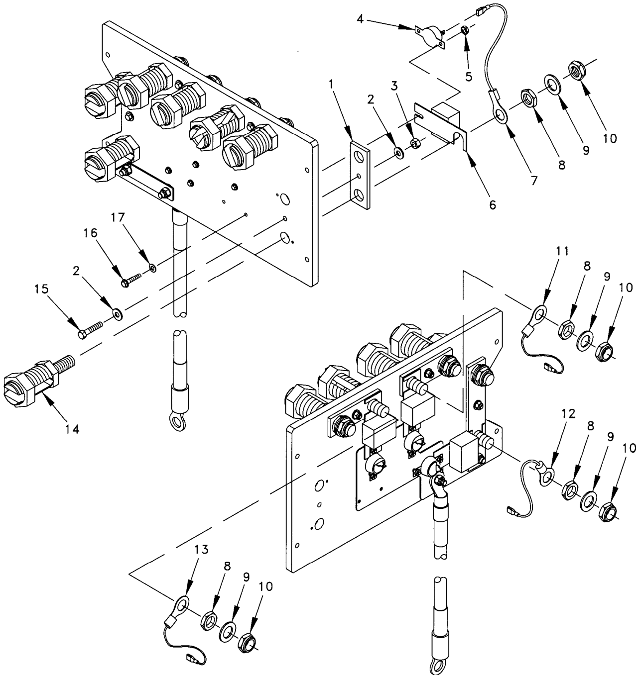
Figure 11. Load Terminal Board Assembly (Sheet 1 of 2).
