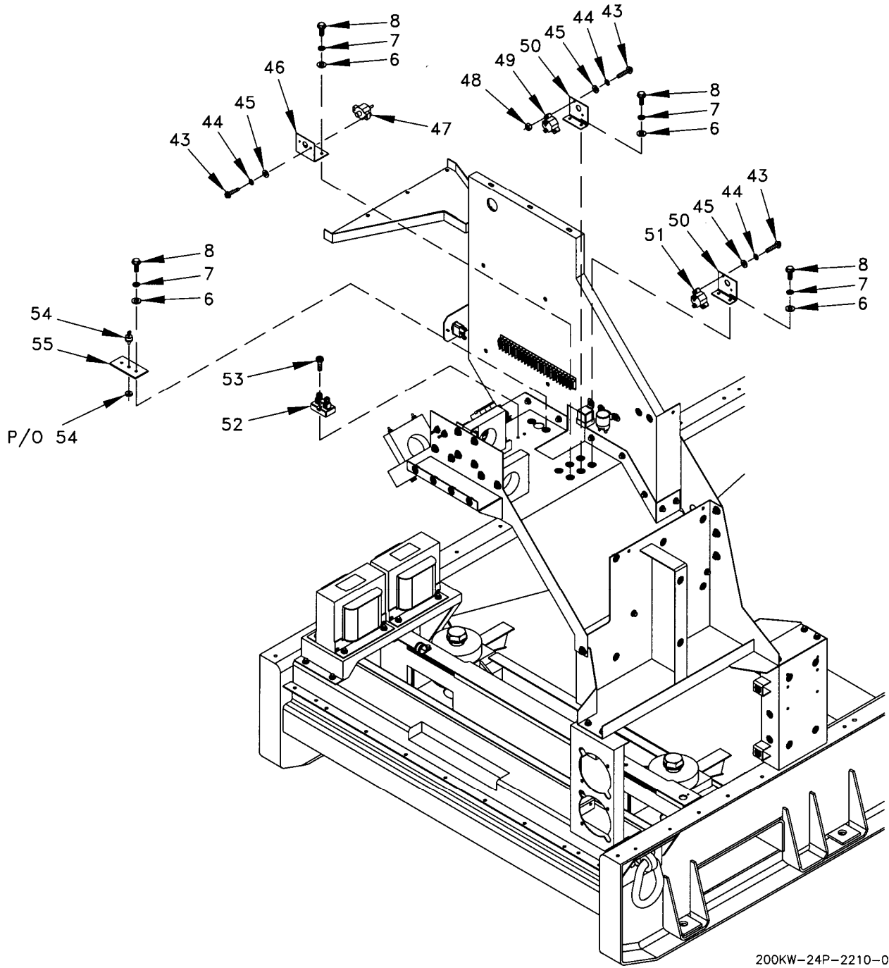
Figure 7. Electrical Components Installation (Sheet 3 of 9).
