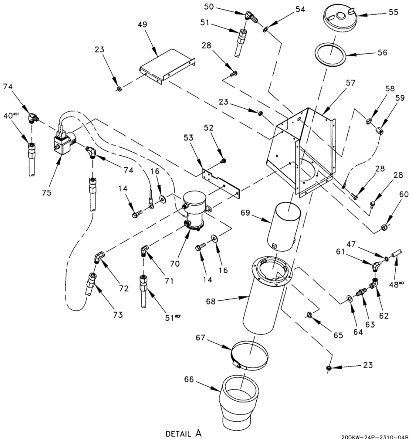
Figure 12. Fuel System Installation (Sheet 4 of 4).
