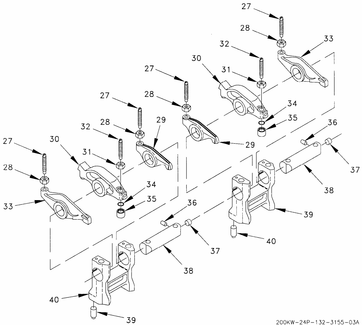
Figure 47. Valve Mounting Group (Sheet 3 of 4).
