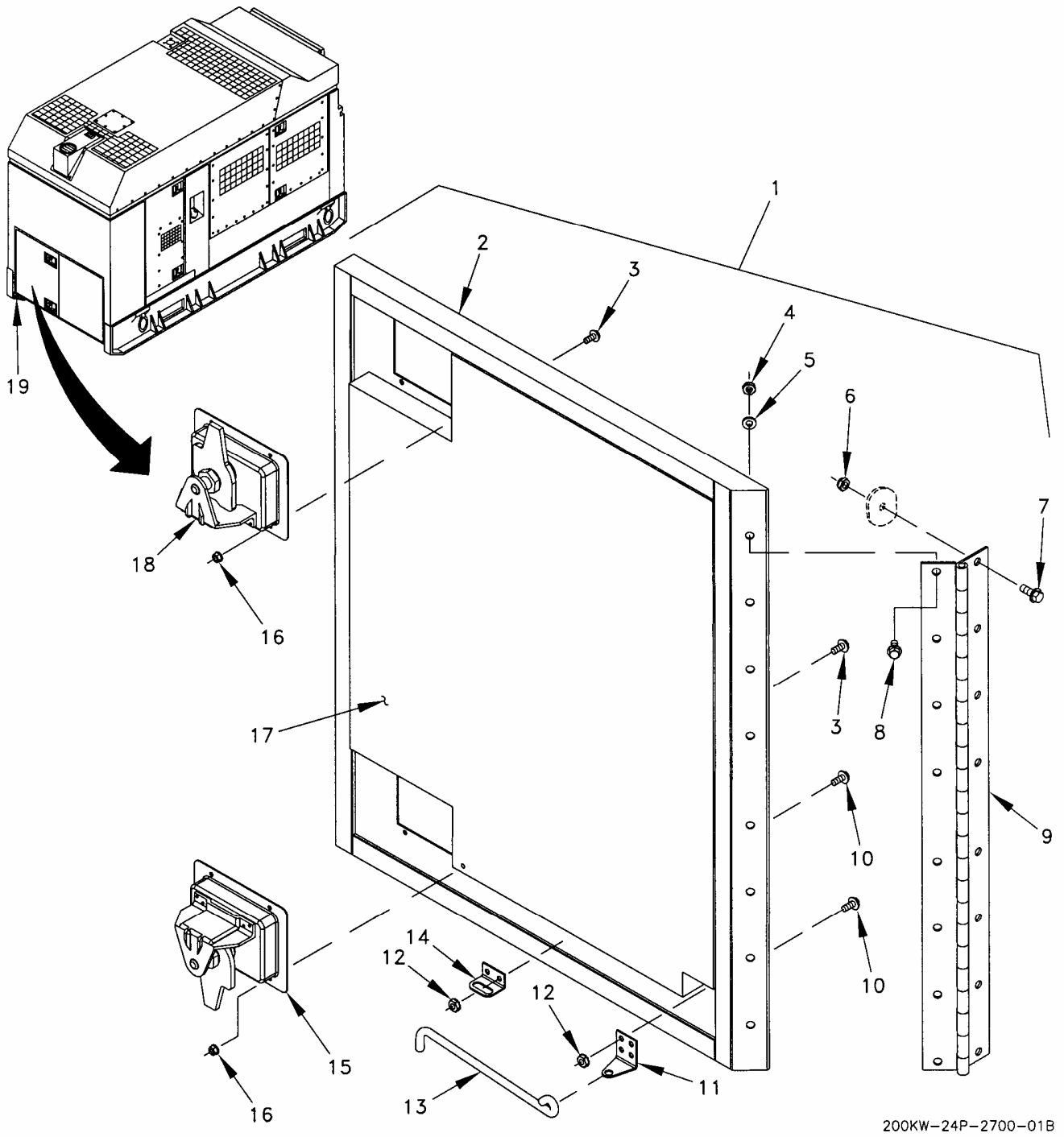
Figure 3. Housing Installation (Sheet 1 of 27).
