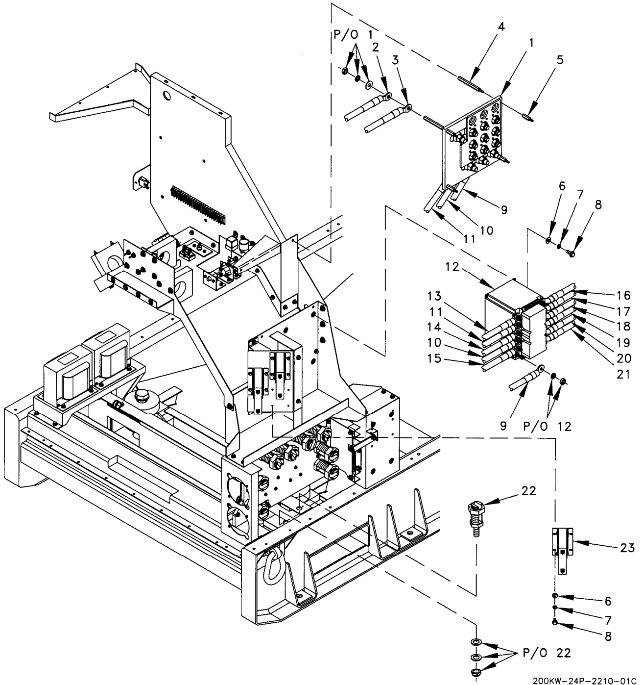
Figure 7. Electrical Components Installation (Sheet 1 of 9).
