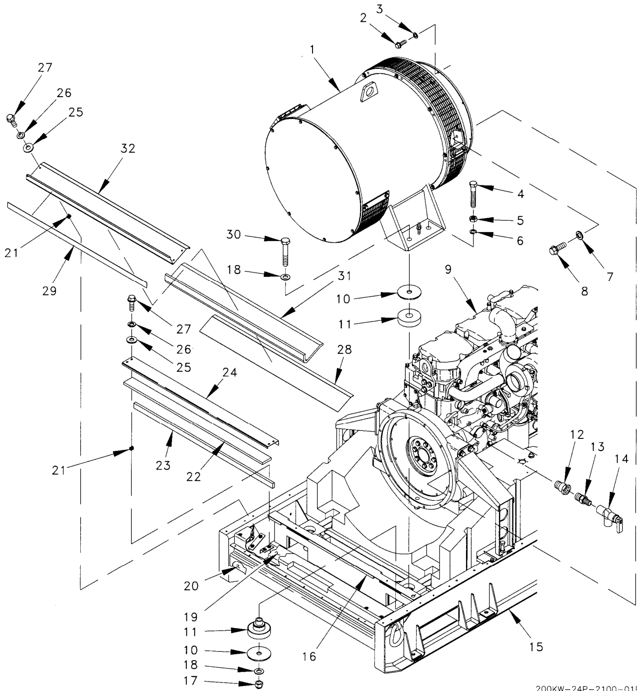
Figure 16. Engine Generator Base Assembly (Sheet 1 of 4).
