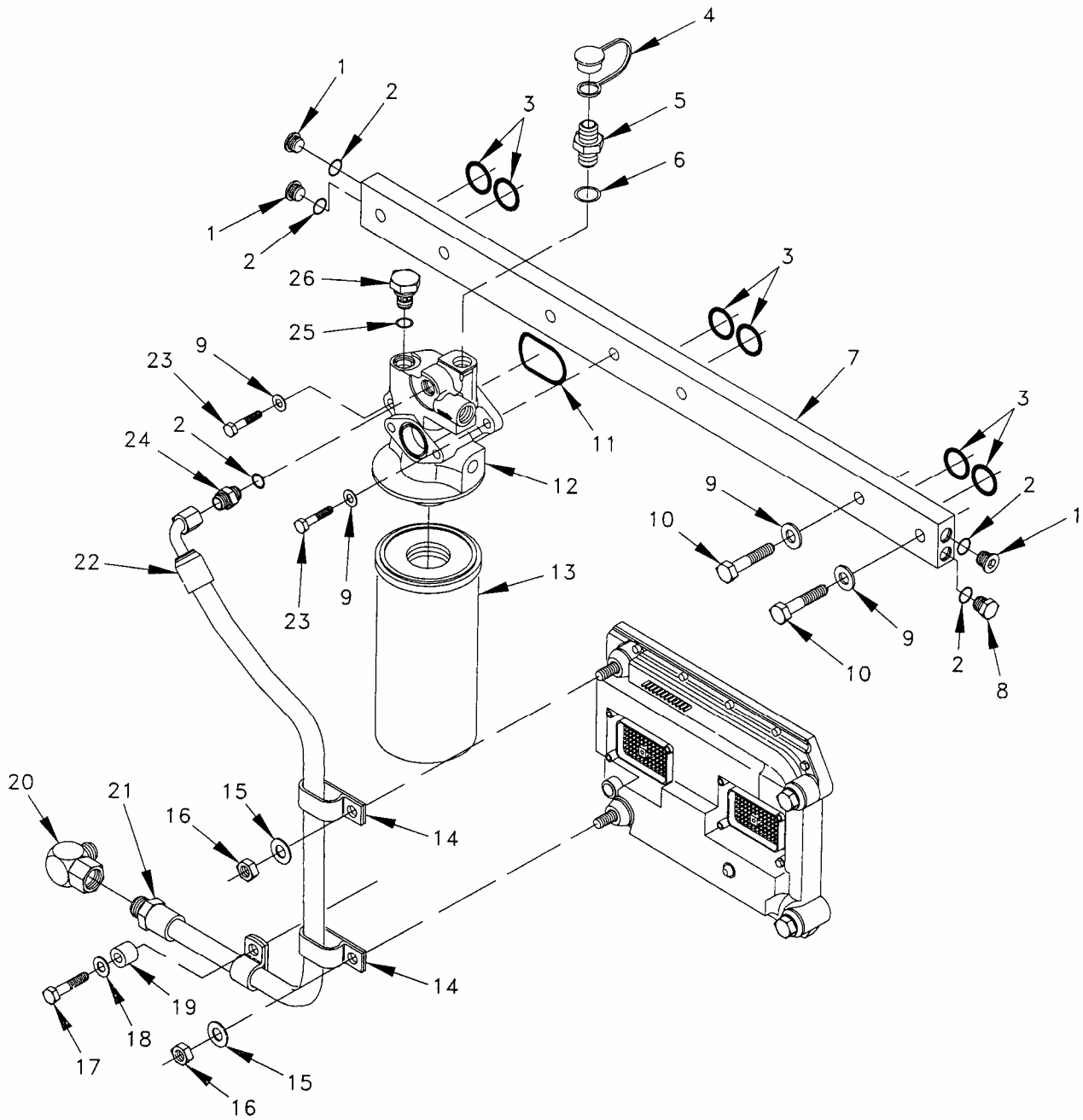
Figure 43. Injection Fuel Group.
