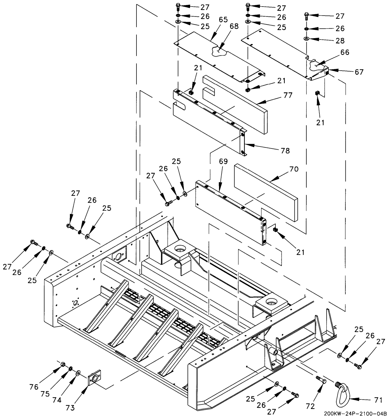
Figure 16. Engine Generator Base Assembly (Sheet 4 of 4).
