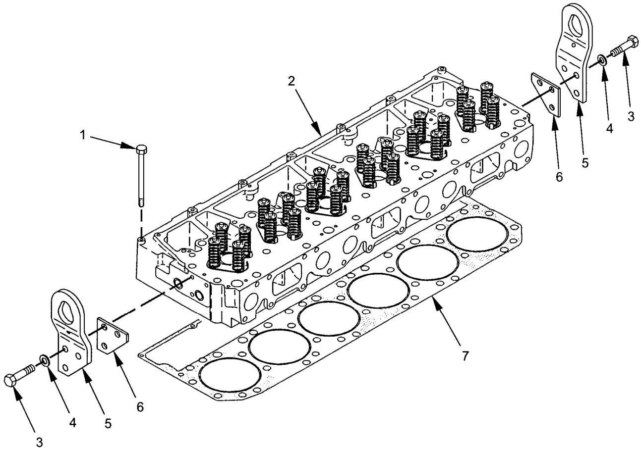
Figure 48. Cylinder Head Group (Sheet 1 of 2).
