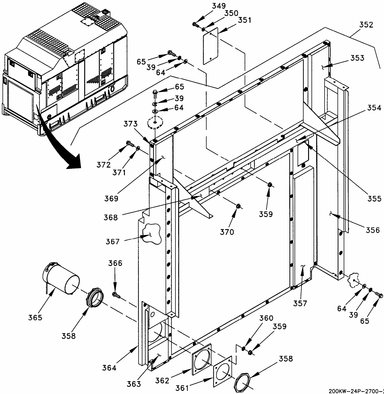
Figure 3. Housing Installation (Sheet 27 of 27).
