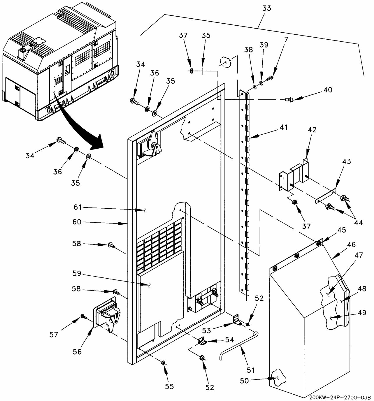
Figure 3. Housing Installation (Sheet 3 of 27).
