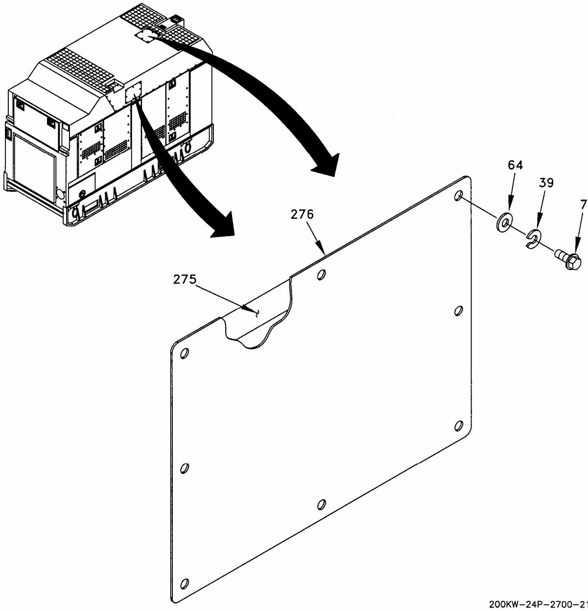
Figure 3. Housing Installation (Sheet 21 of 27).
