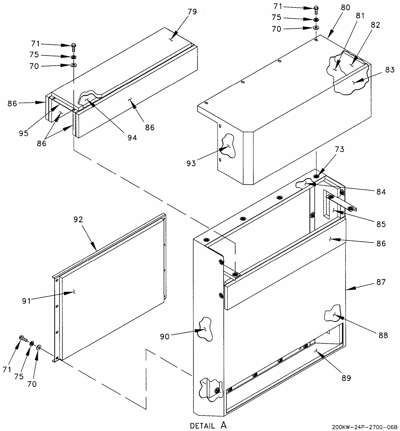
Figure 3. Housing Installation (Sheet 6 of 27).
