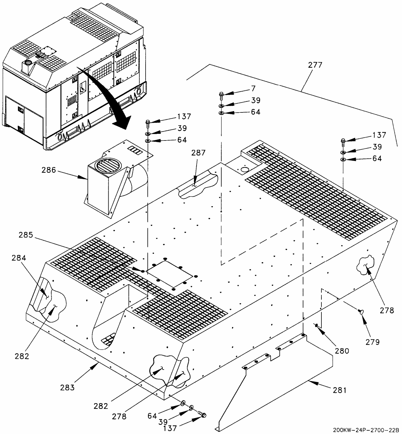
Figure 3. Housing Installation (Sheet 22 of 27).
