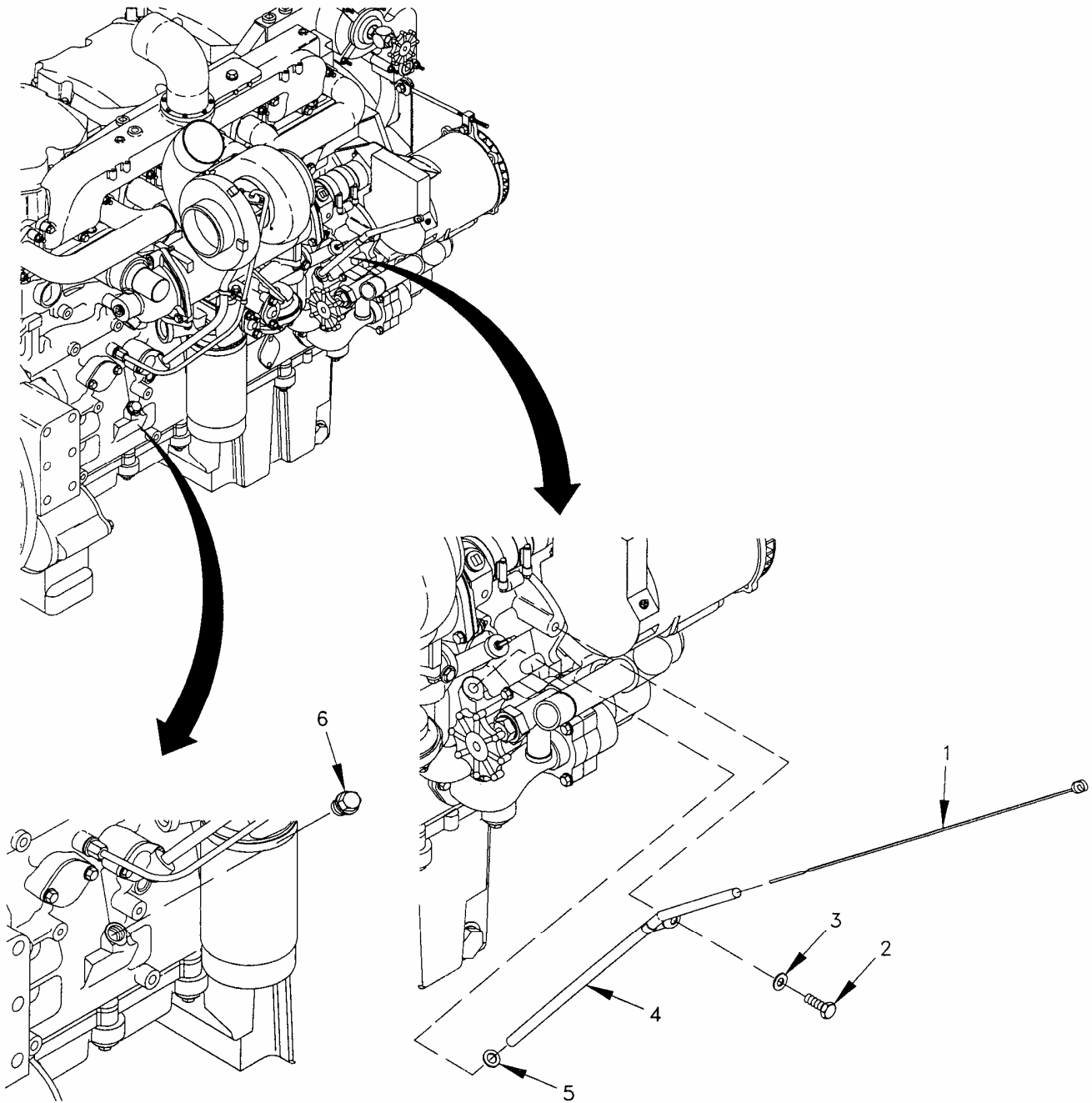
Figure 40. Oil Gage Group.
