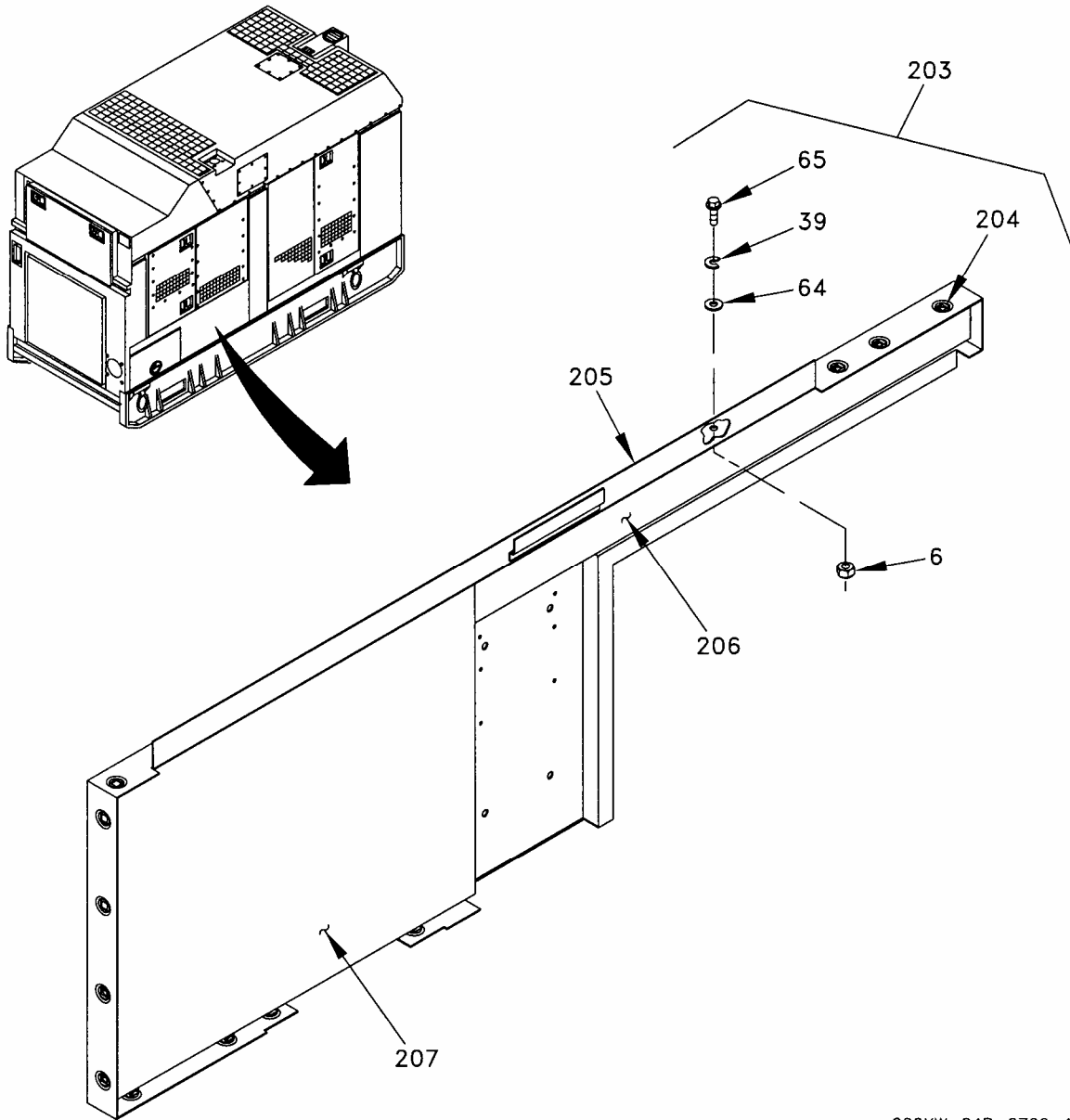
Figure 3. Housing Installation (Sheet 16 of 27).
