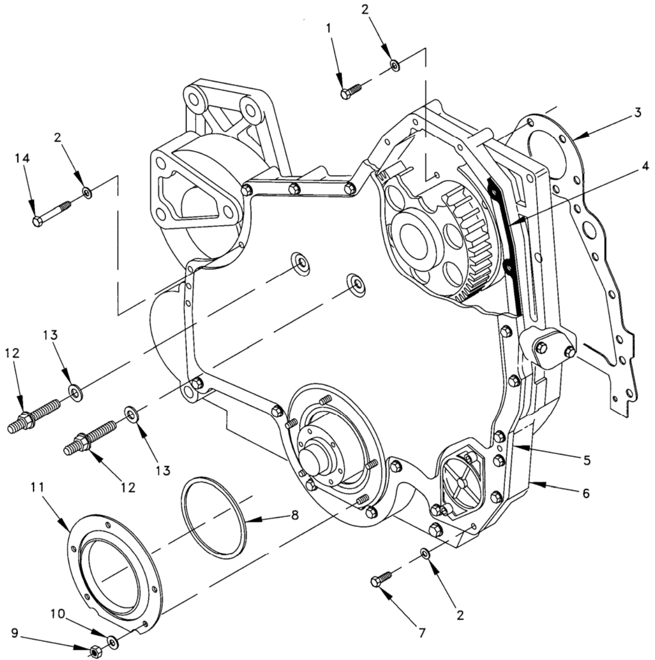
Figure 55. Front Housing Group.
