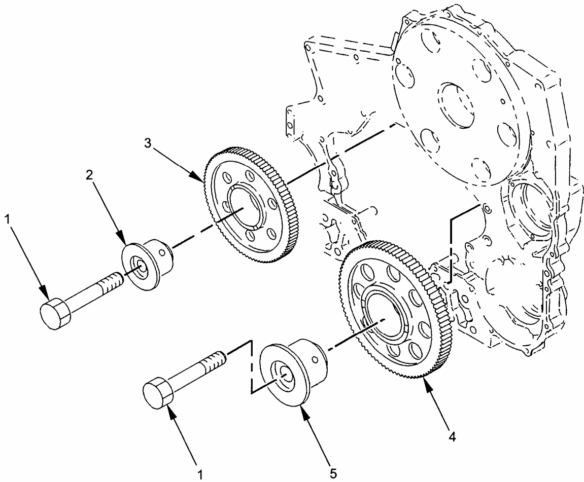
Figure 56. Front Gear Group.
