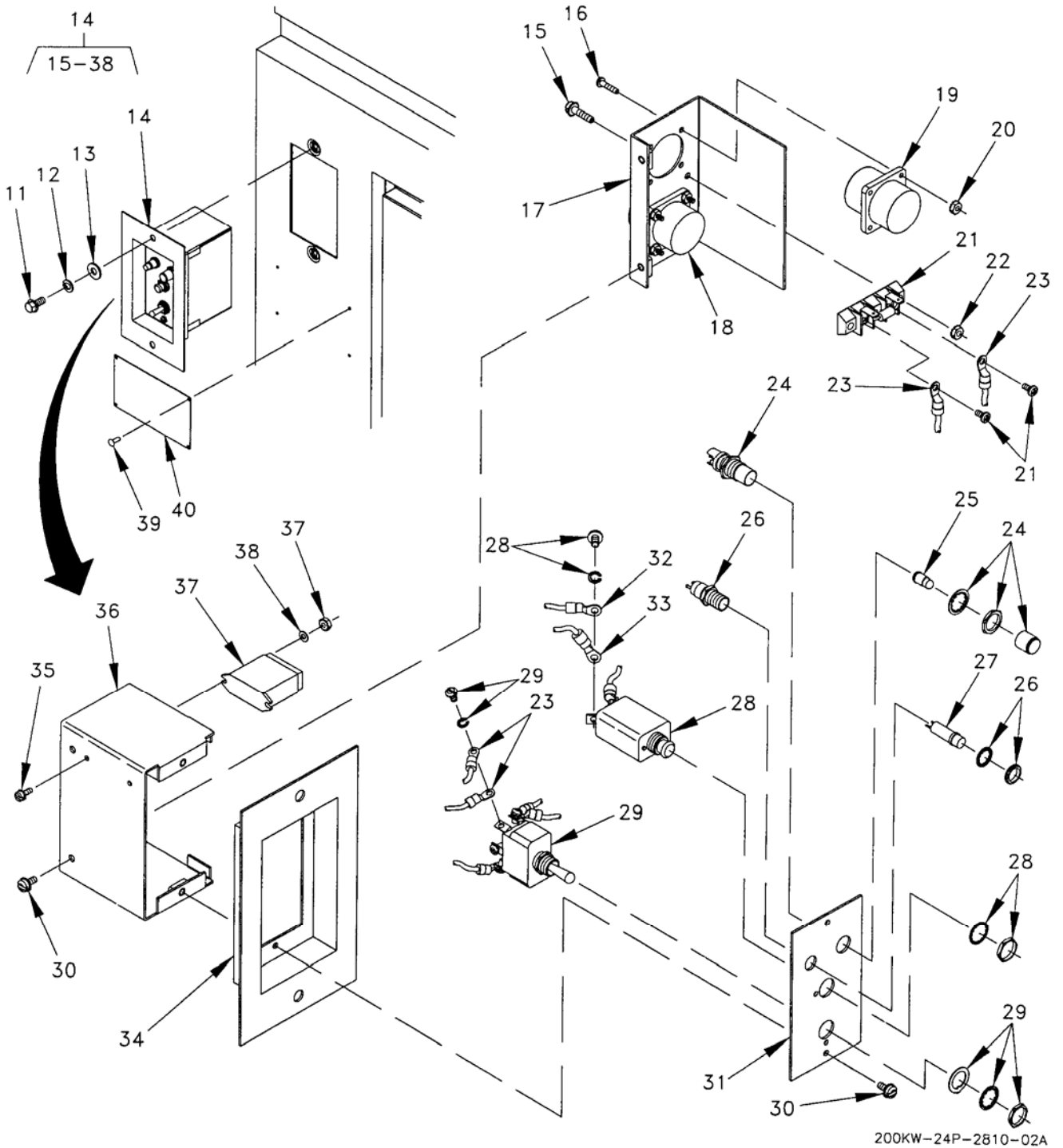
Figure 60. Winterization Group (Sheet 2 of 5).
