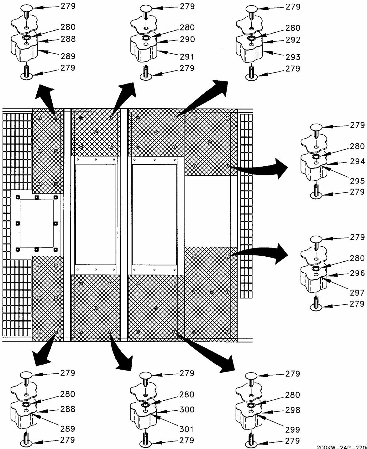
Figure 3. Housing Installation (Sheet 23 of 27).
