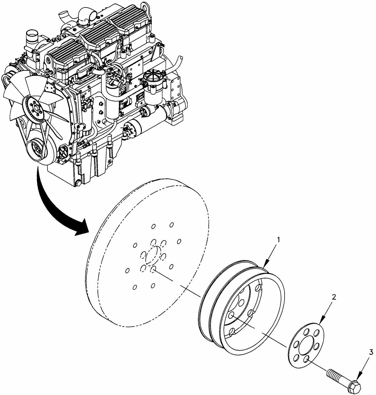
Figure 51. Crankshaft Pulley Group.
