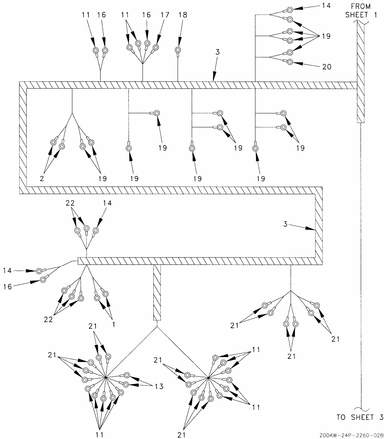
Figure 9. Engine Harness Assembly (Sheet 2 of 3).
