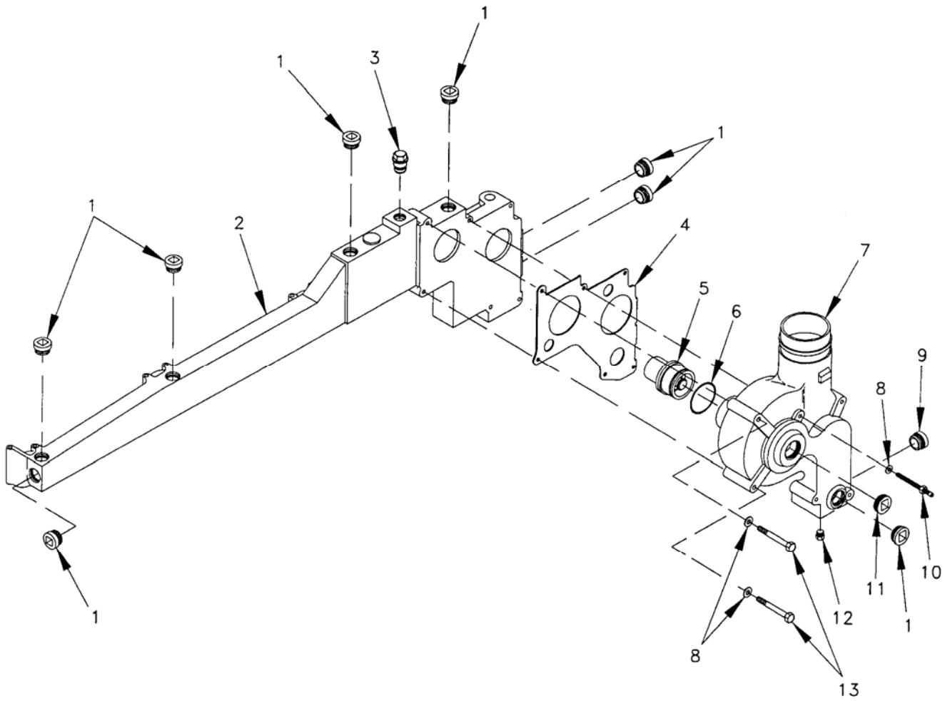
Figure 24. Water Regulator Housing Group.
