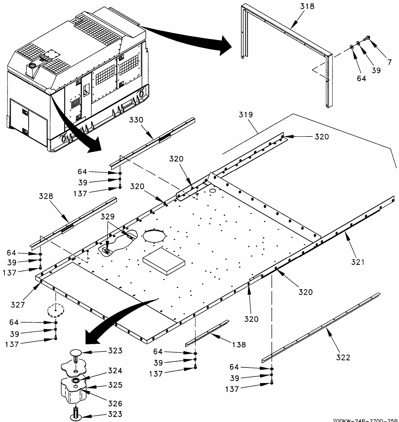
Figure 3. Housing Installation (Sheet 25 of 27).
