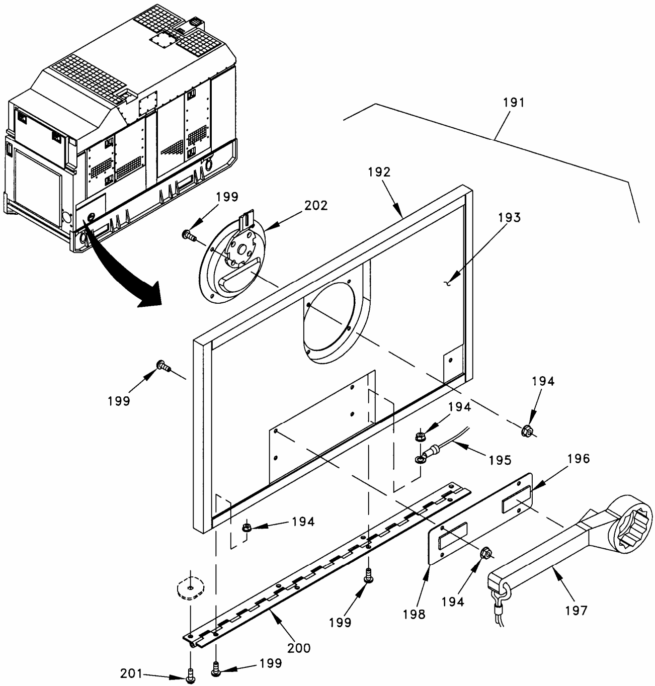
Figure 3. Housing Installation (Sheet 15 of 27).
