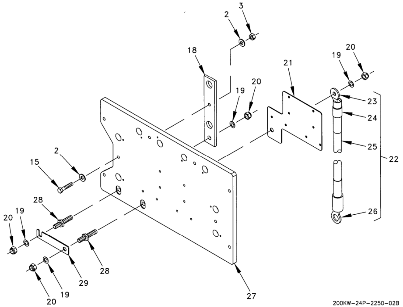
Figure 11. Load Terminal Board Assembly (Sheet 2 of 2).
