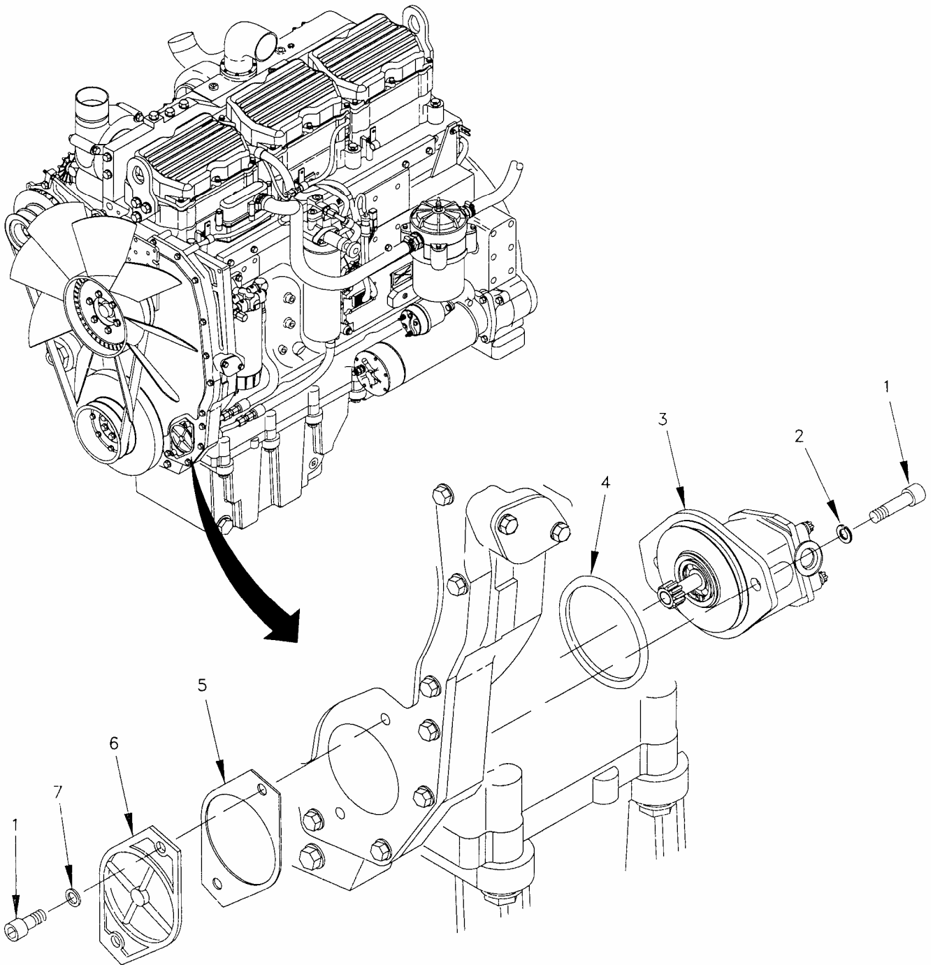
Figure 45. Fuel Transfer Group.
