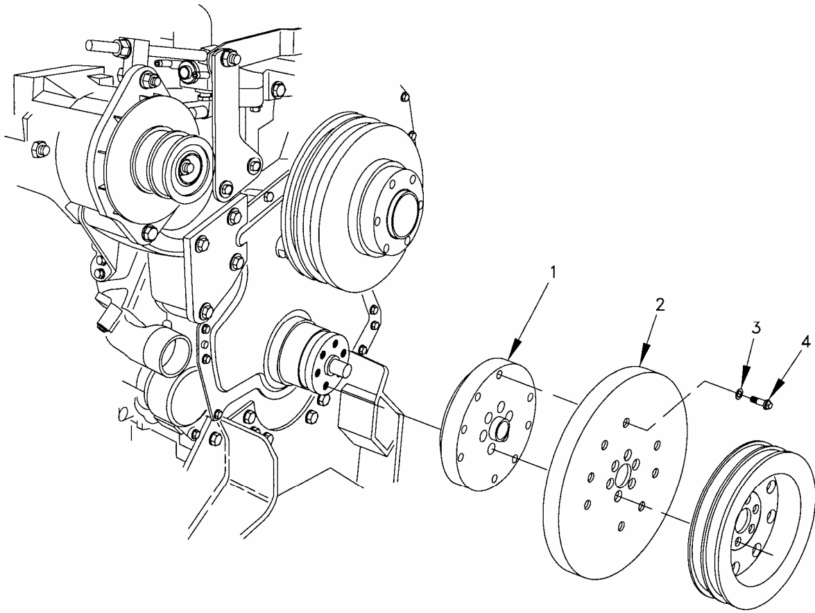
Figure 52. Crankshaft Damper Group.
