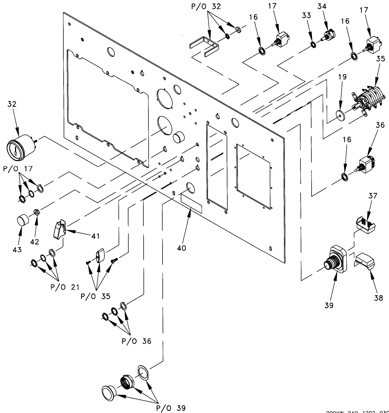
Figure 6. Control Box Panel Assembly (Sheet 3 of 3).
