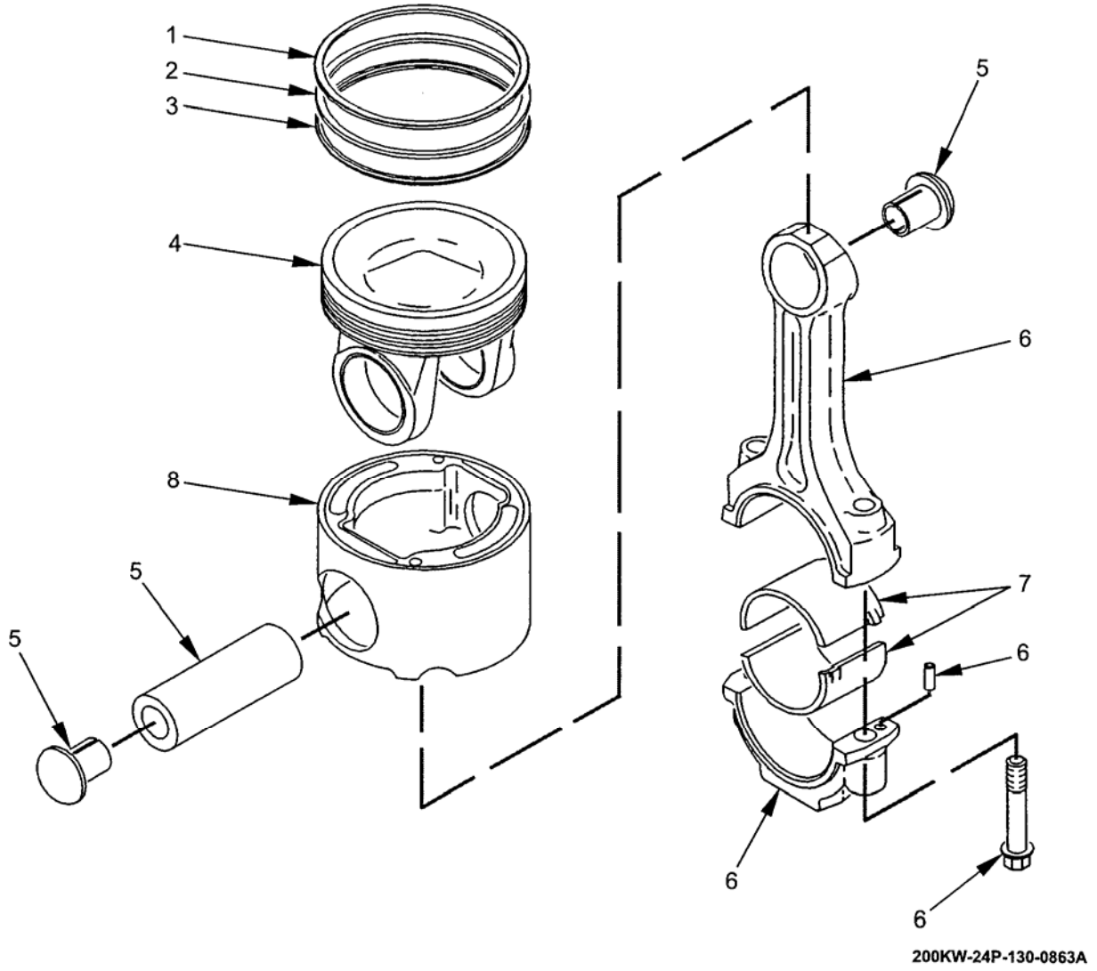
Figure 58. Piston Group.
