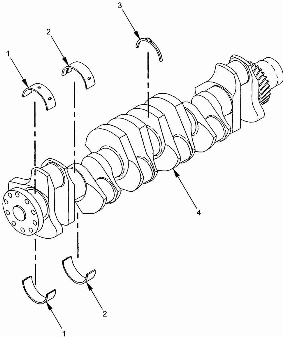
Figure 54. Crankshaft Group.
