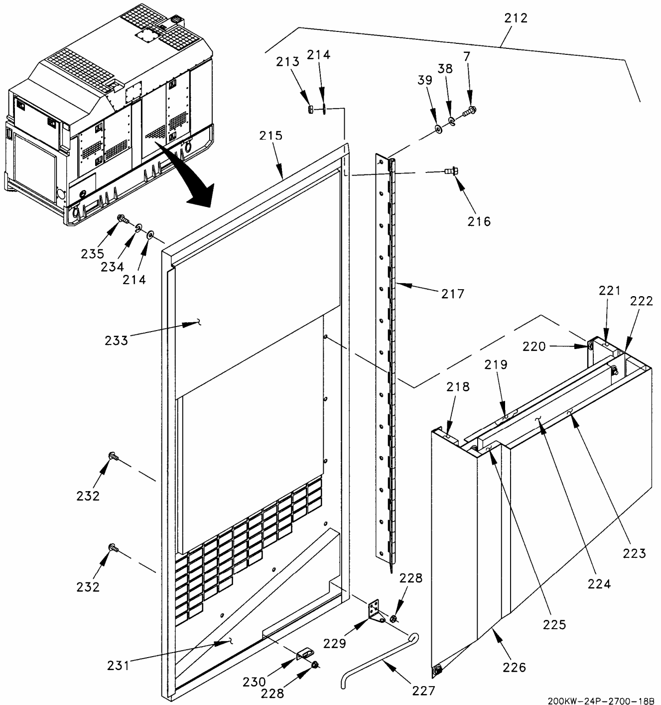
Figure 3. Housing Installation (Sheet 18 of 27).
