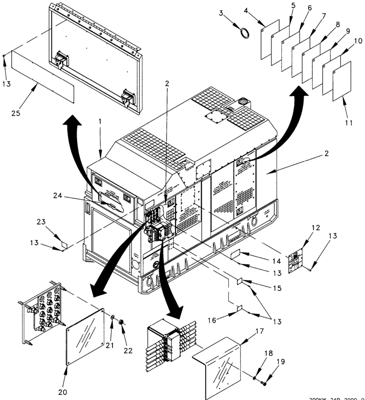
Figure 1. Generator Set, Tactical Quiet, 200 kW, 50/60 Hz (Sheet 1 of 2).
