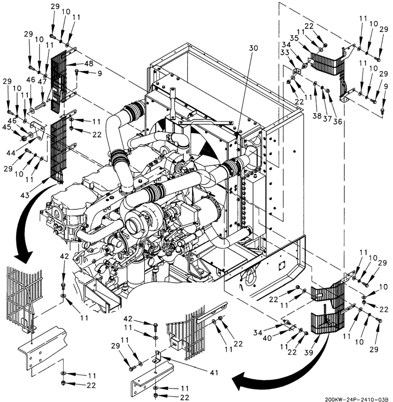
Figure 13. Cooling System Installation (Sheet 3 of 6).
