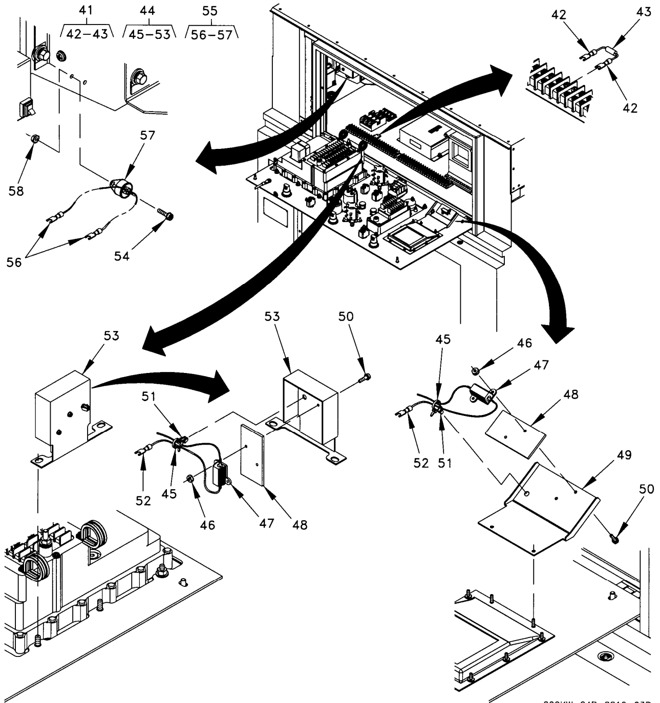
Figure 60. Winterization Group (Sheet 3 of 5).
