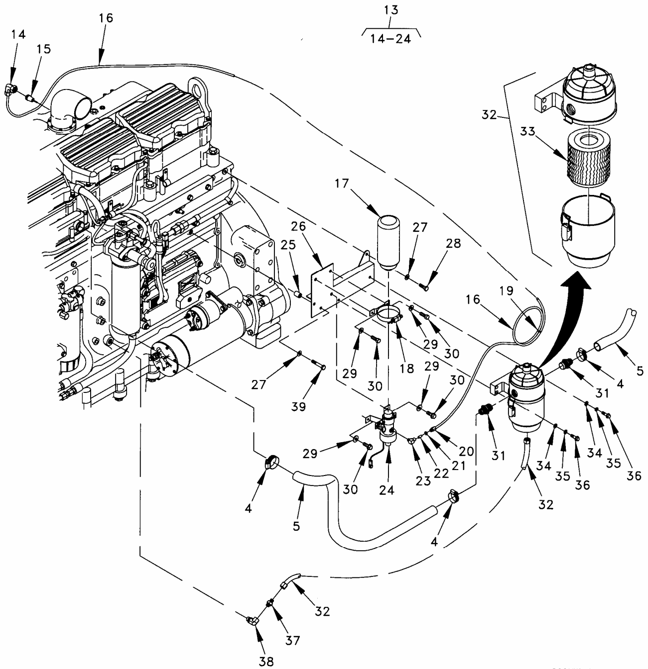
Figure 15. Air Cleaner Installation (Sheet 2 of 3).
