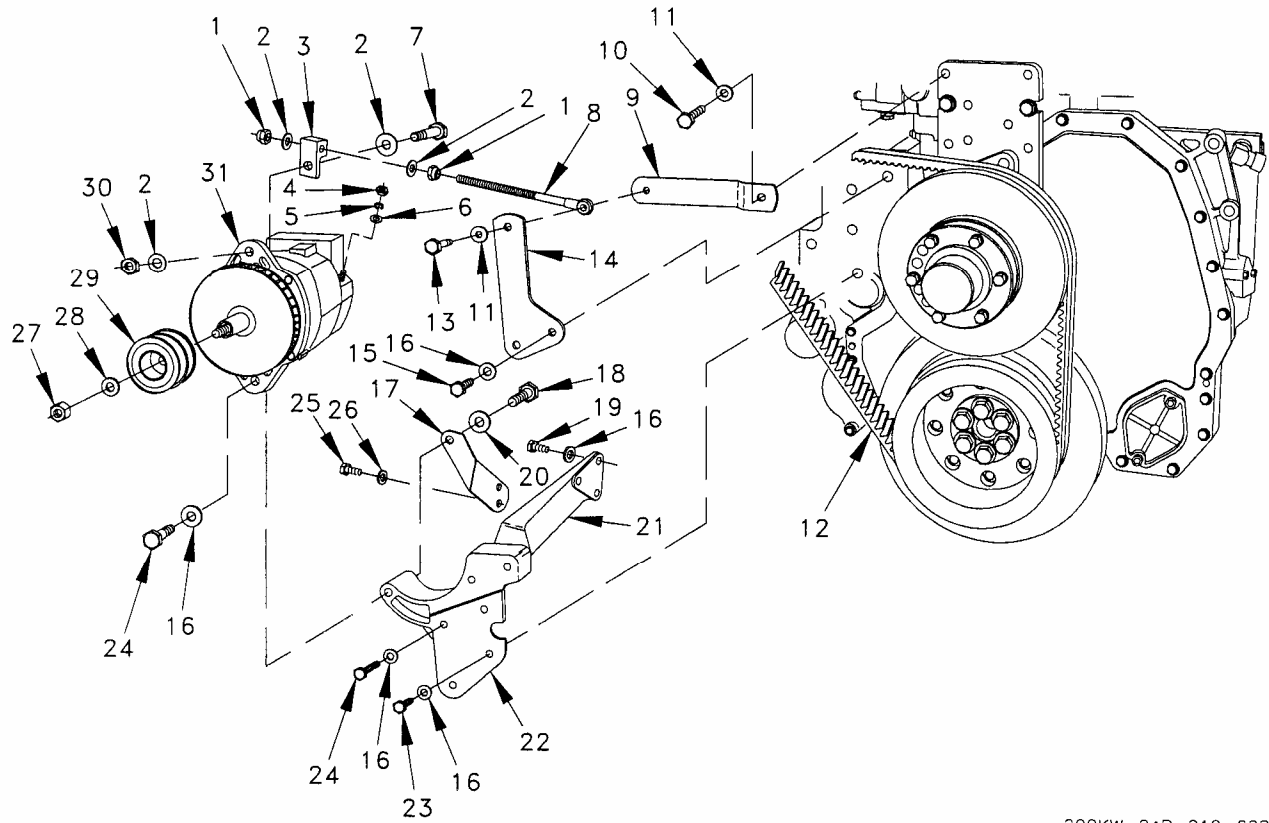
Figure 18. Alternator Mounting Group.
