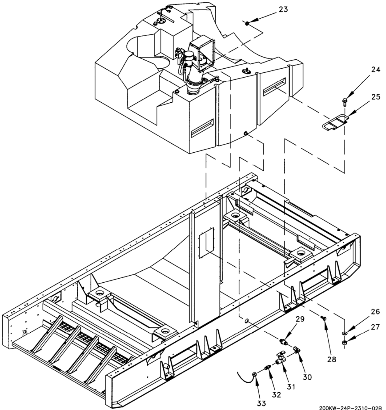
Figure 12. Fuel System Installation (Sheet 2 of 4).
