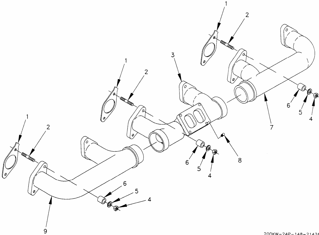
Figure 33. Exhaust Manifold Group.
