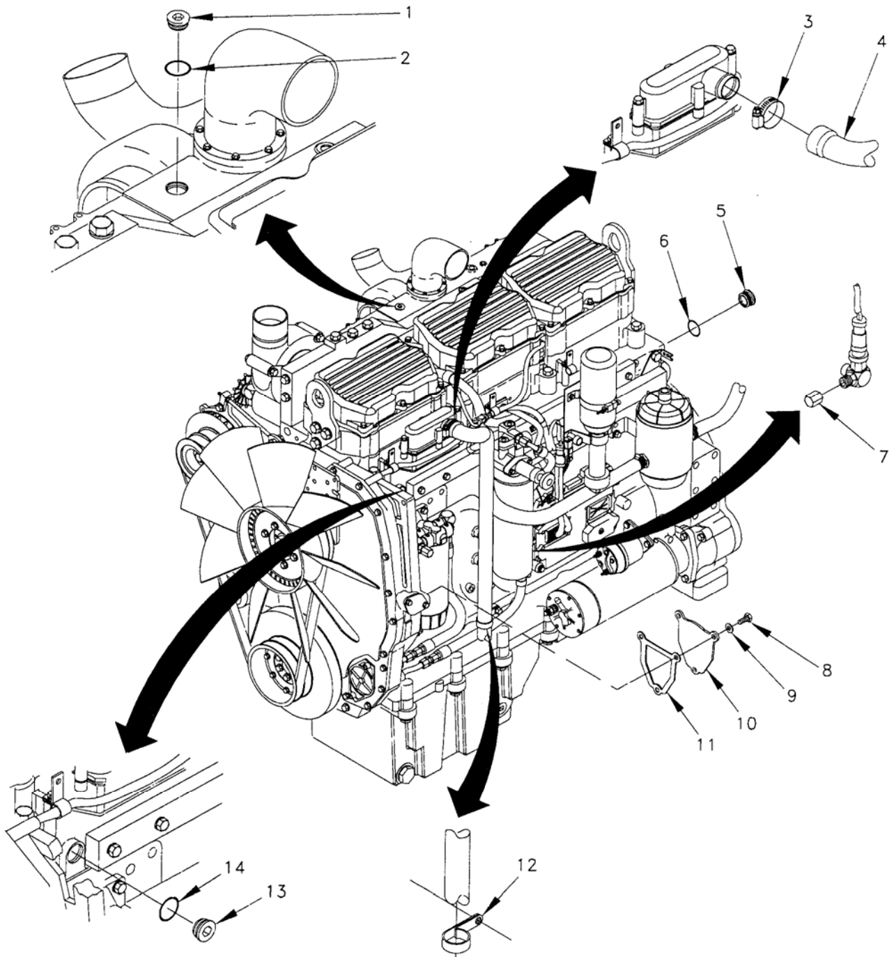
Figure 26. Air Compressor Cover Group.
