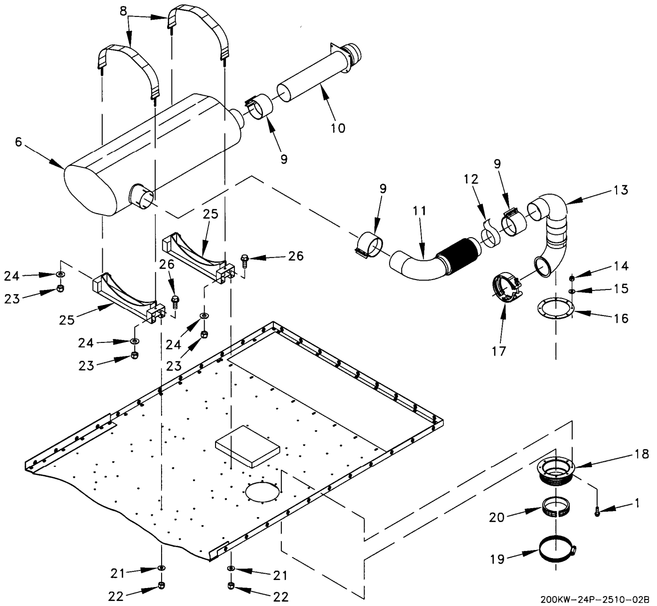
Figure 14. Exhaust System Installation (Sheet 2 of 2).
