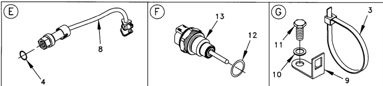
Figure 29. Electronic Control Wiring Group (Sheet 1 of 4).
