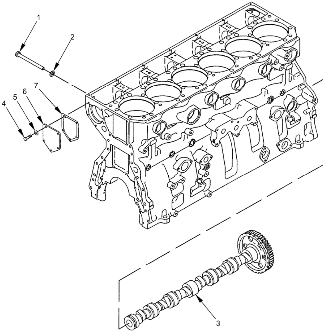
Figure 57. Camshaft Group.
