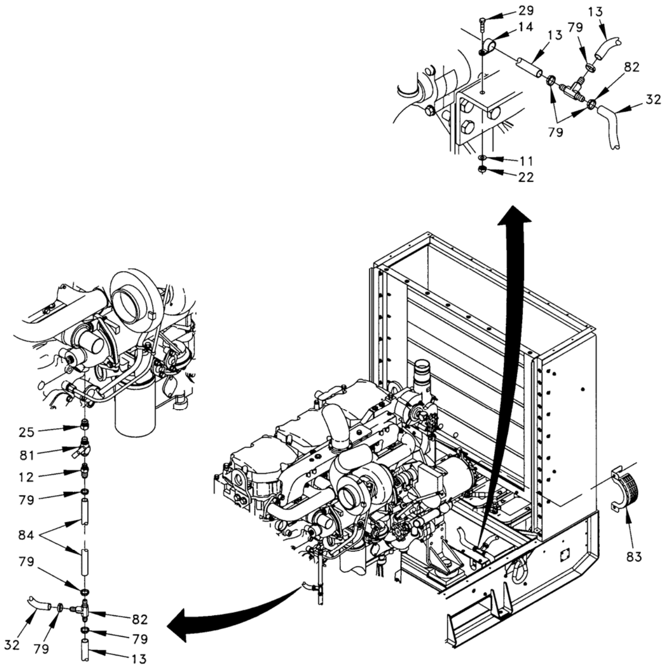
Figure 13. Cooling System Installation (Sheet 5 of 6).
