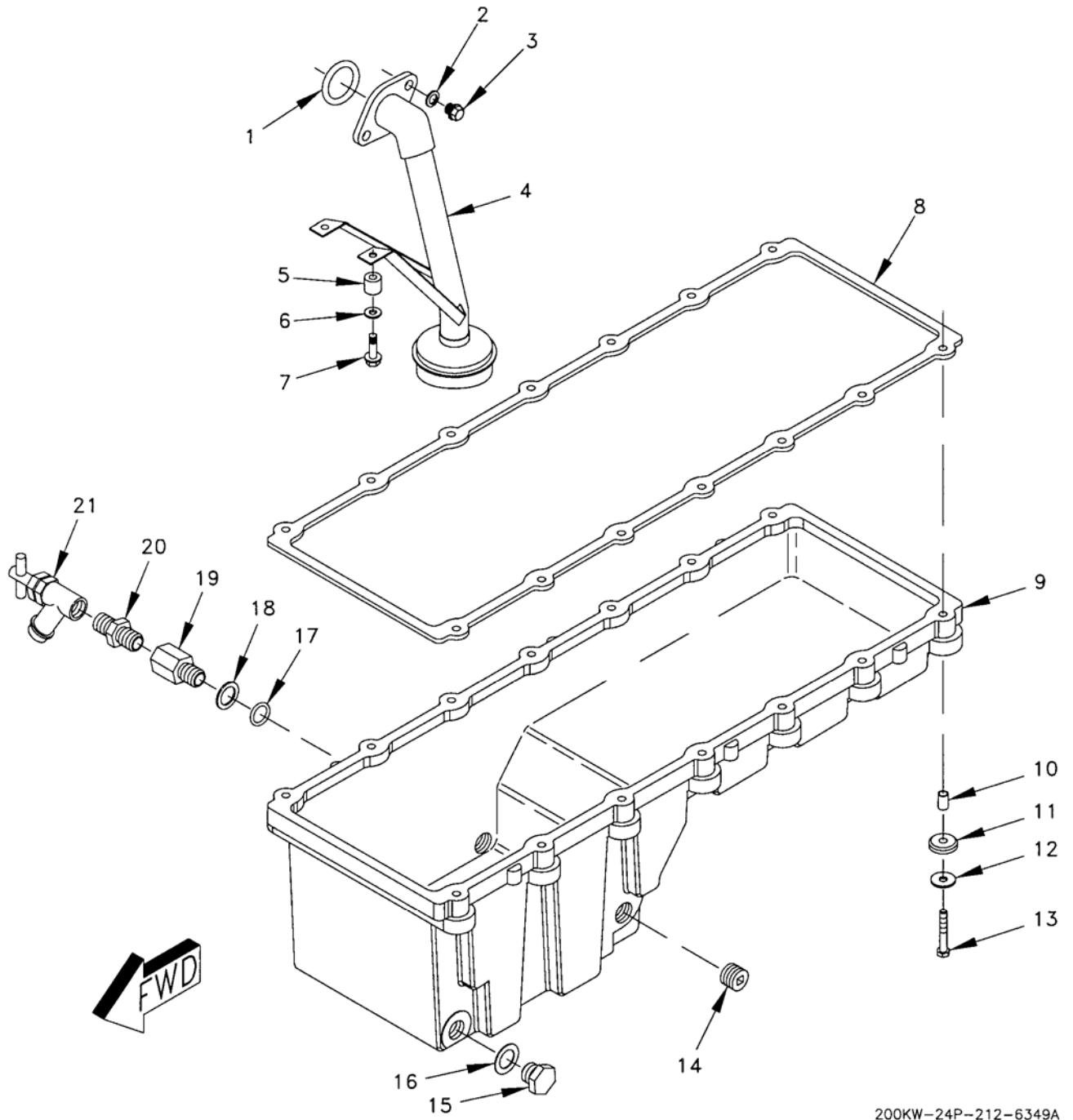
Figure 35. Oil Pan Group.
