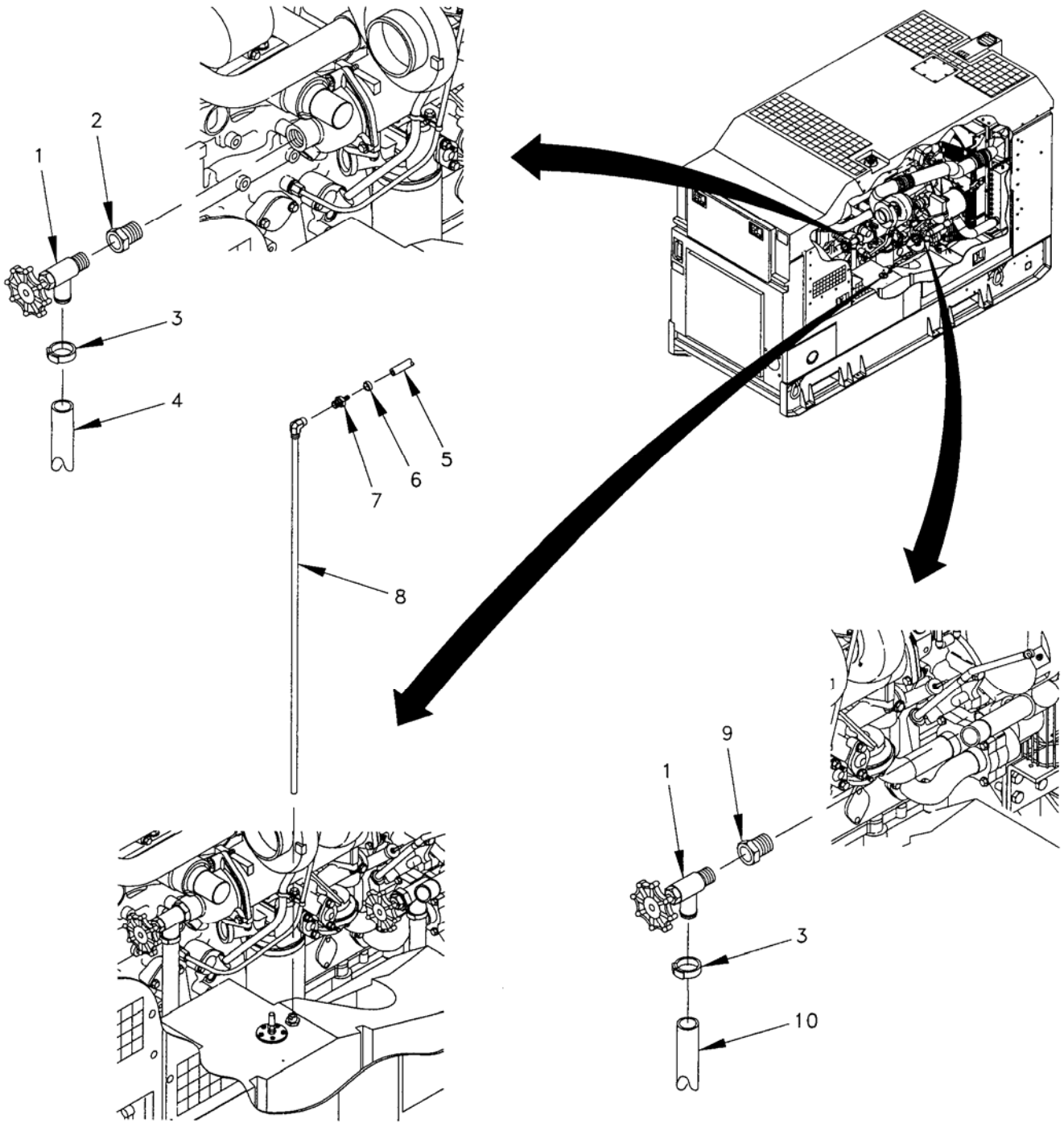
Figure 60. Winterization Group (Sheet 1 of 5).
