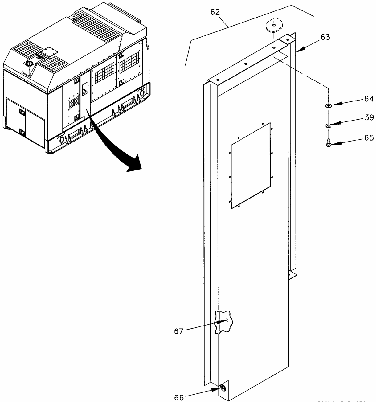
Figure 3. Housing Installation (Sheet 4 of 27).
