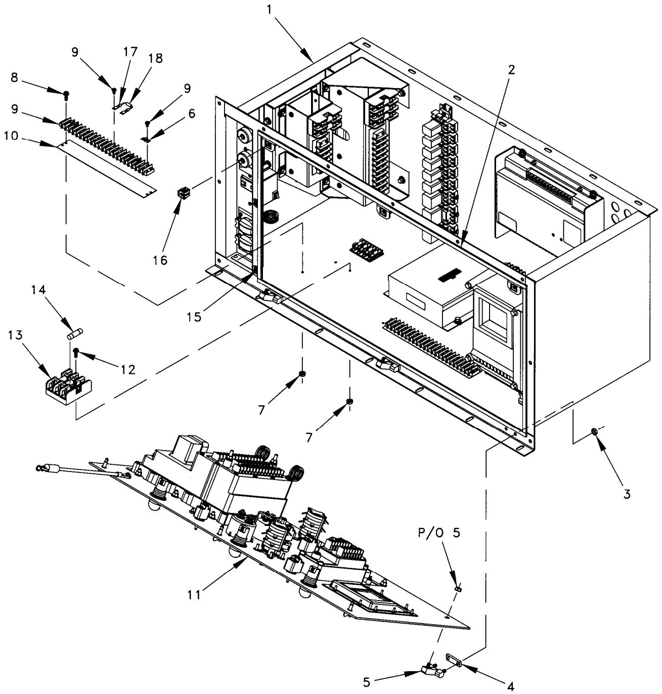
Figure 4. Control Box Assembly (Sheet 1 of 5).
