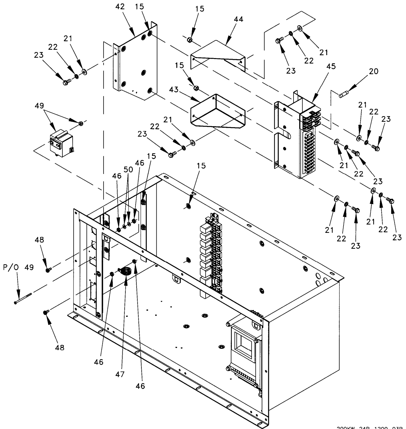
Figure 4. Control Box Assembly (Sheet 3 of 5).
