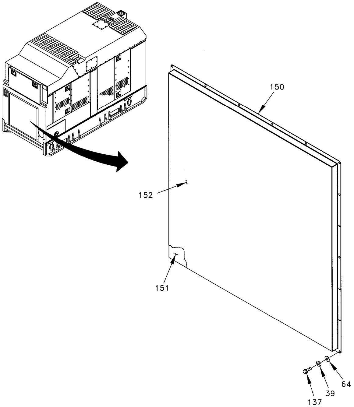
Figure 3. Housing Installation (Sheet 12 of 27).
