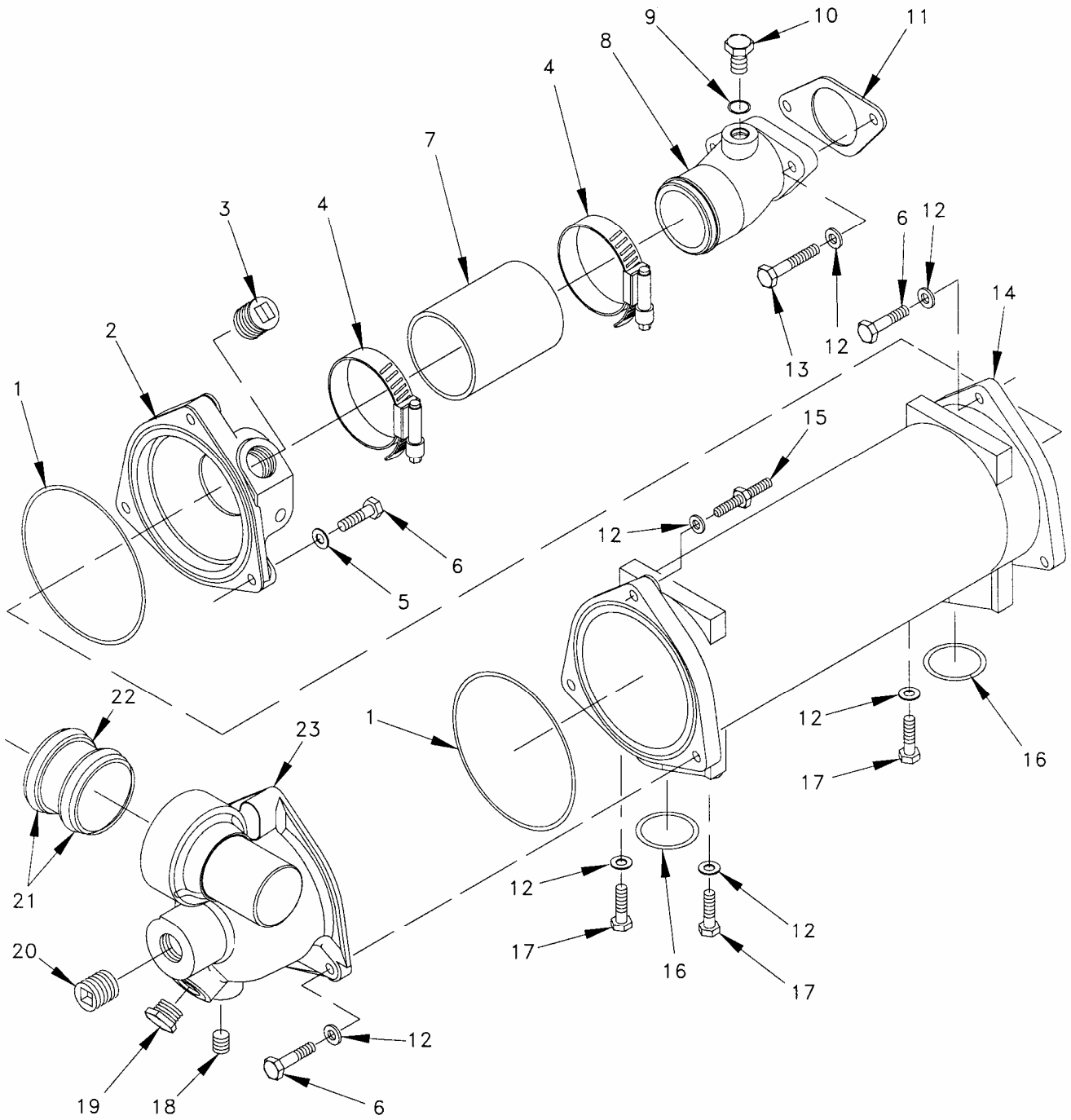
Figure 38. Oil Cooler Group.
