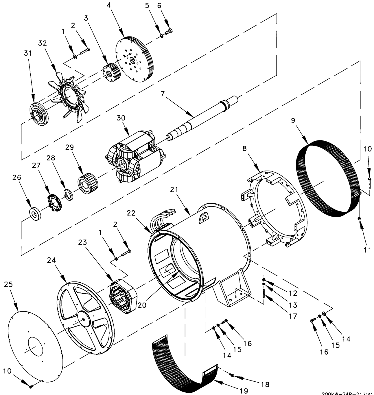
Figure 17. Generator.
