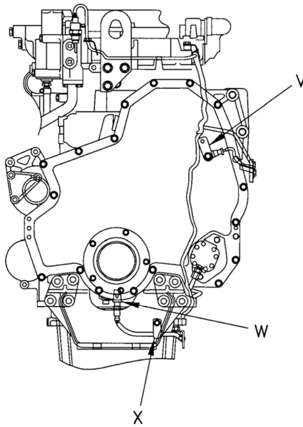
Figure 29. Electronic Control Wiring Group (Sheet 4 of 4).
