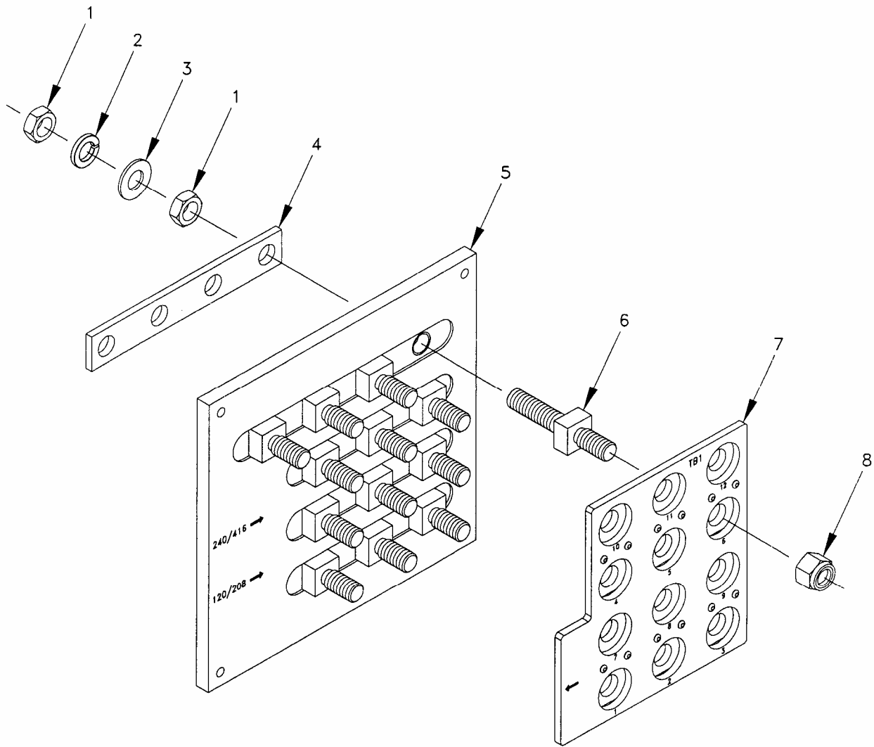
Figure 10. Reconnection Board Assembly.
