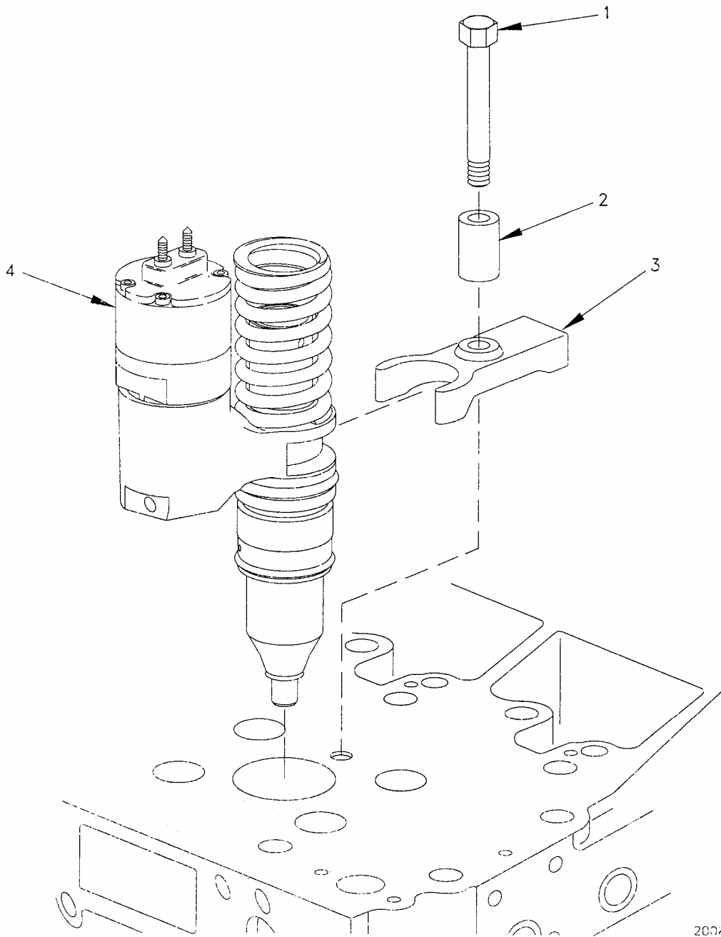
Figure 46. Fuel Injection Group.
