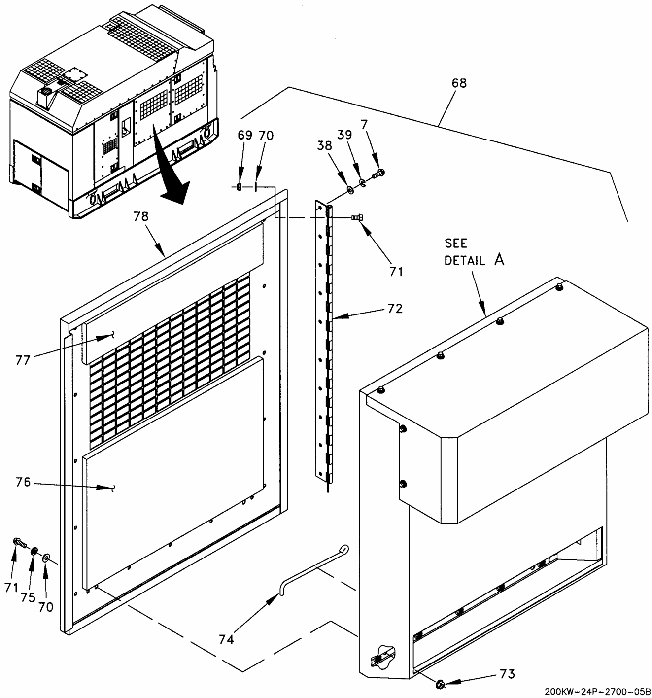
Figure 3. Housing Installation (Sheet 5 of 27).
