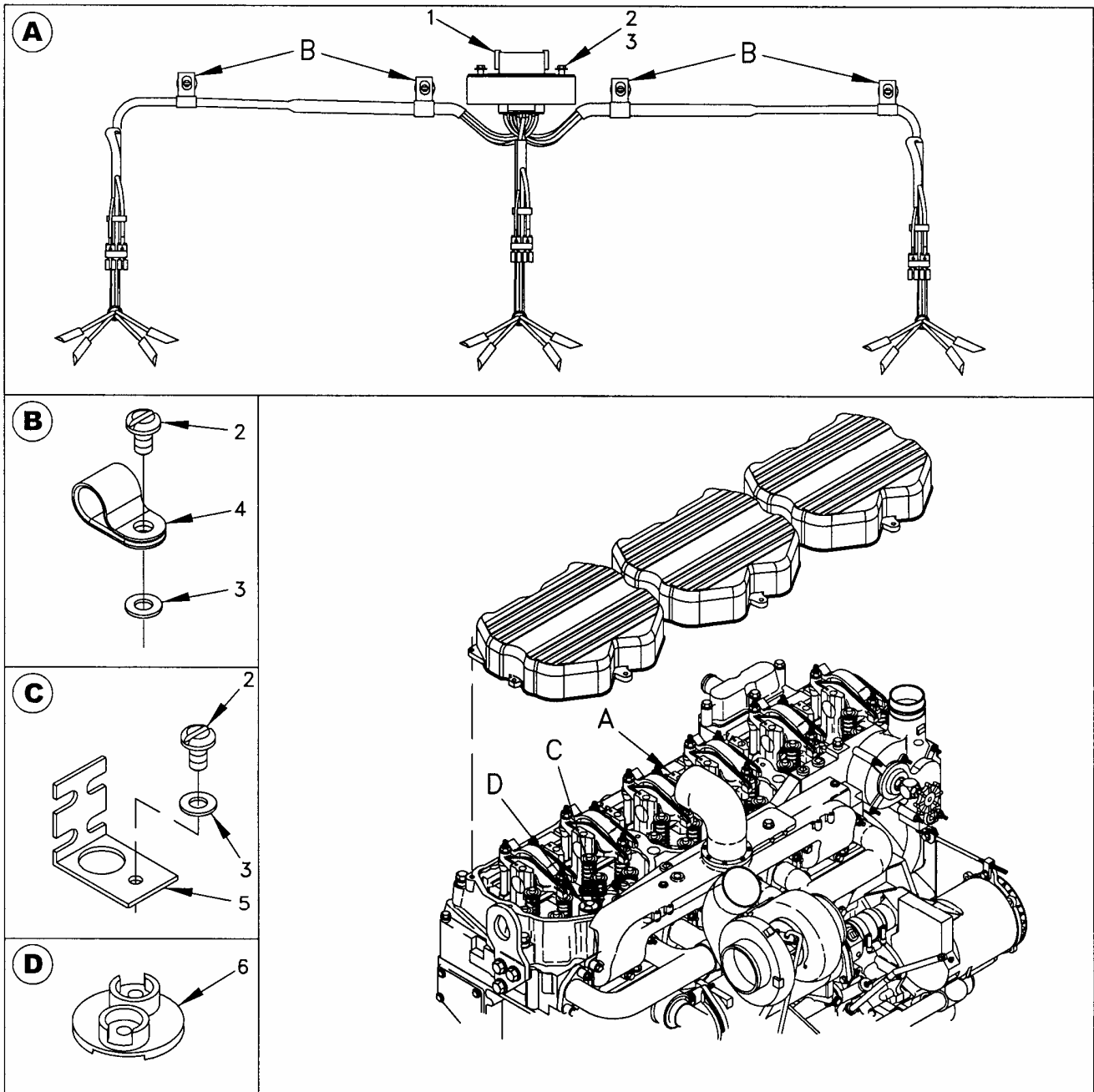
Figure 30. Injector Unit Wiring Group.
