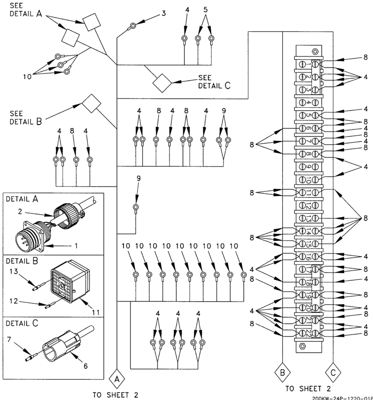
Figure 5. Control Box Harness Assembly (Sheet 1 of 5).
