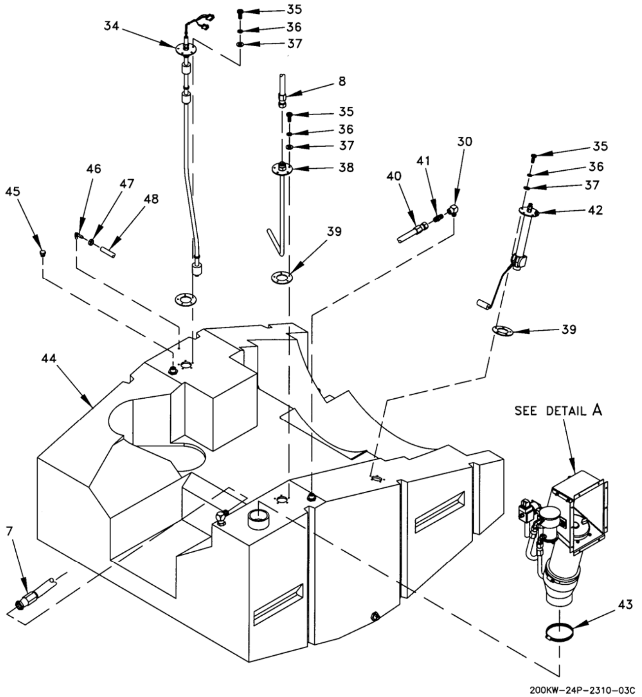
Figure 12. Fuel System Installation (Sheet 3 of 4).
