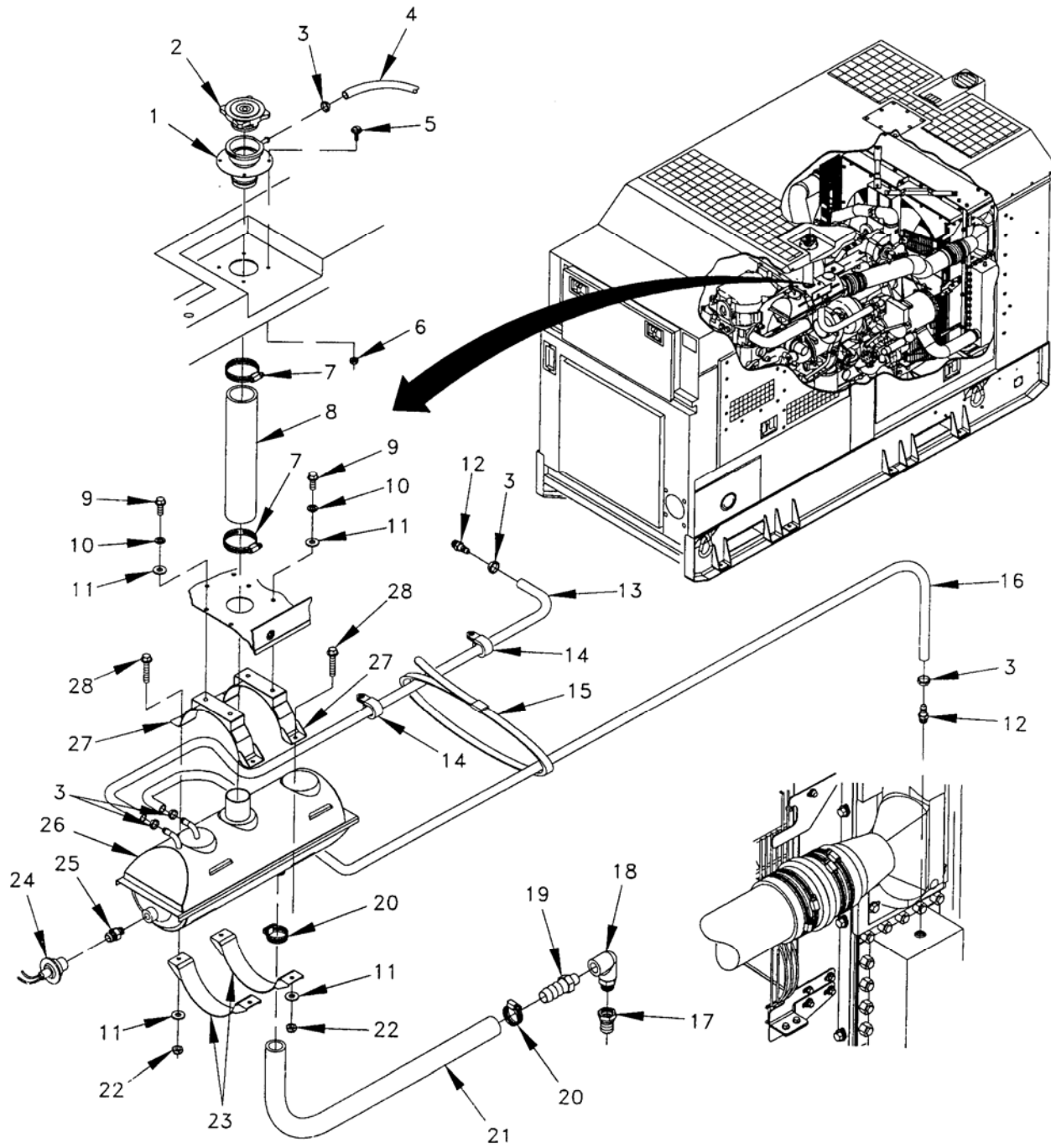
Figure 13. Cooling System Installation (Sheet 1 of 6).
