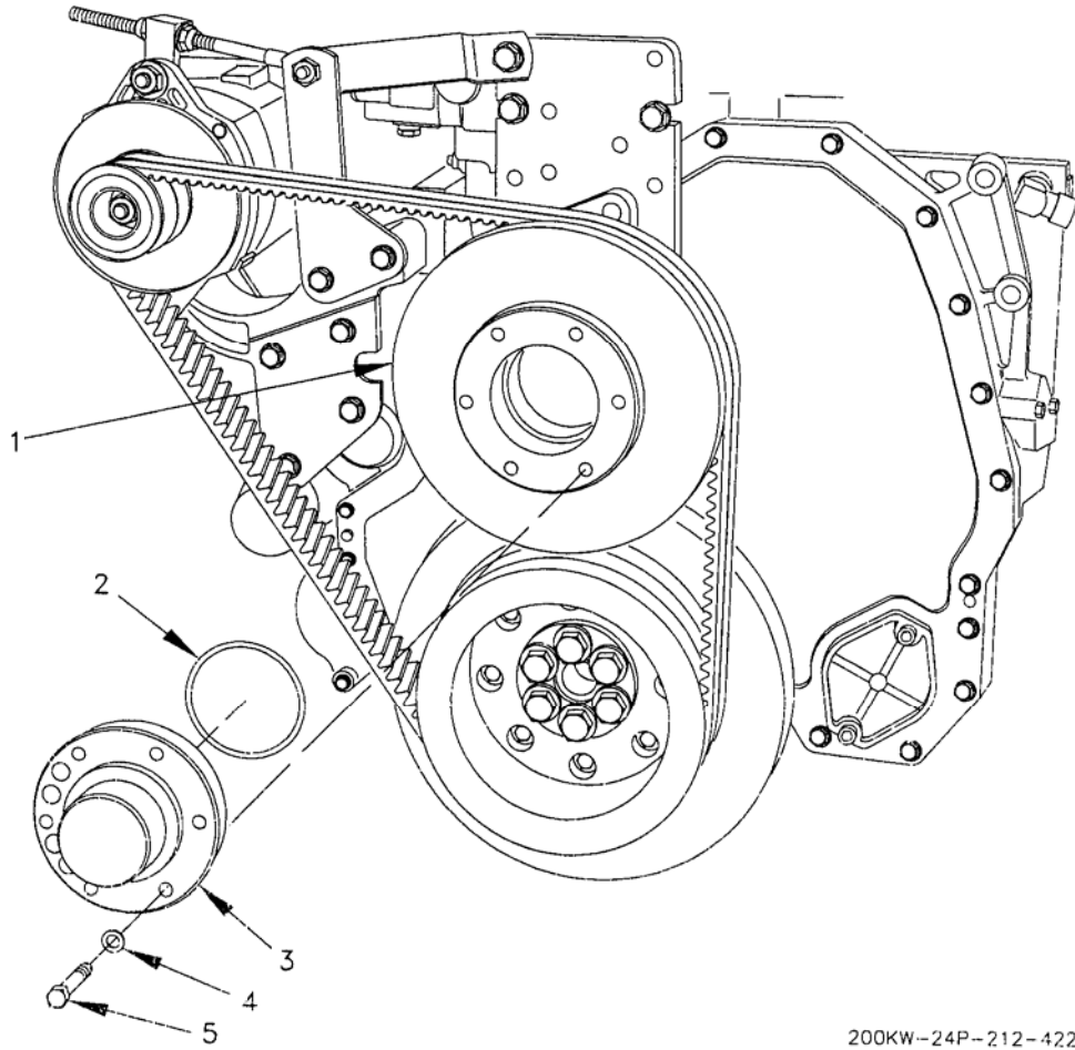
Figure 19. Pulley Group.
