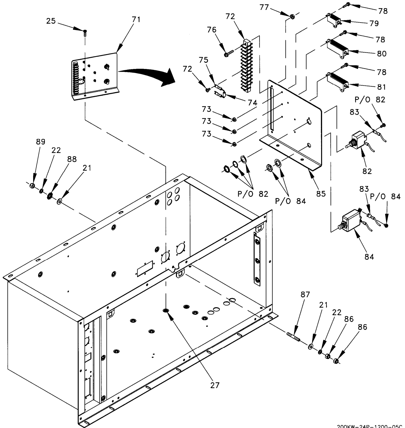
Figure 4. Control Box Assembly (Sheet 5 of 5).
