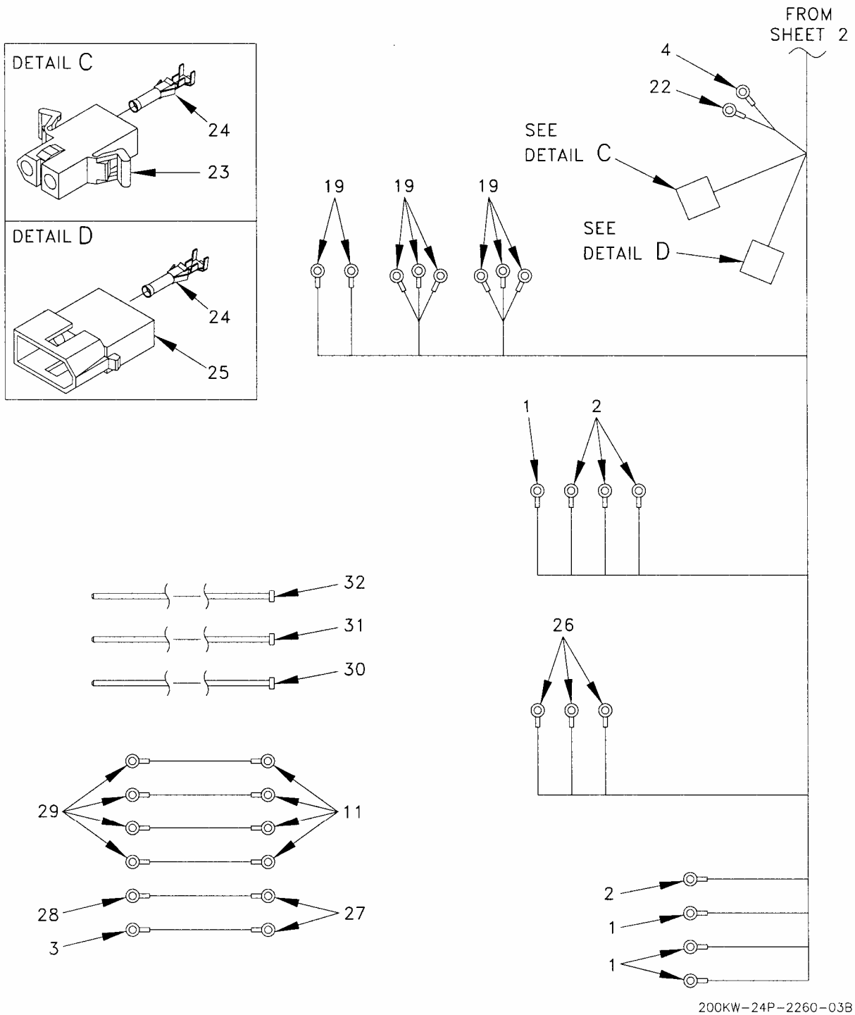
Figure 9. Engine Harness Assembly (Sheet 3 of 3).
