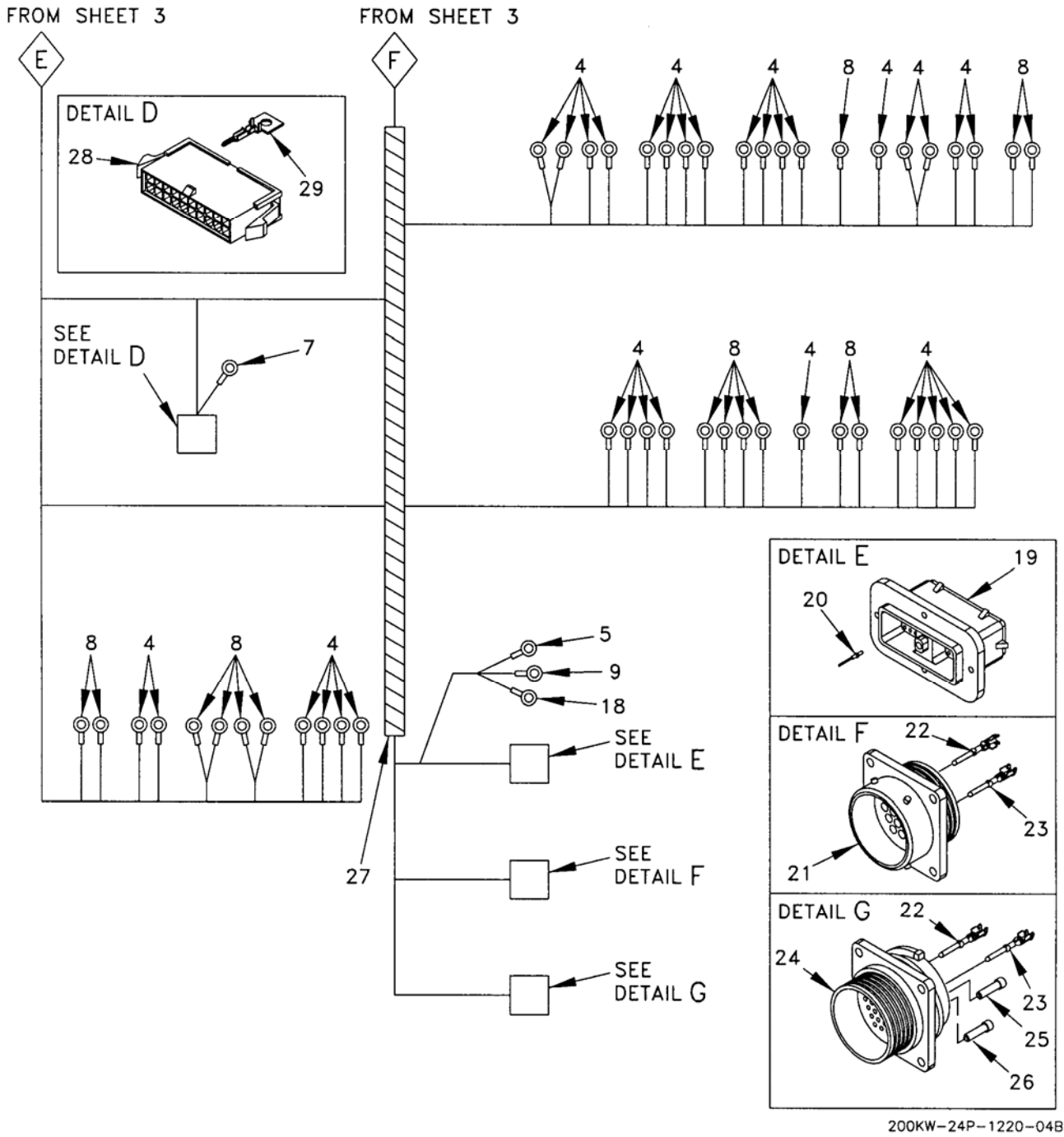
Figure 5. Control Box Harness Assembly (Sheet 4 of 5).
