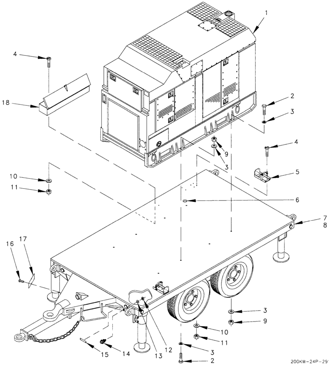
Figure 61. Trailer Installation.
