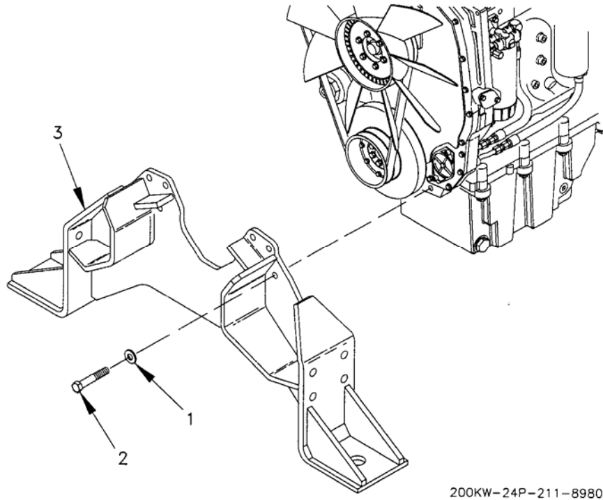
Figure 28. Engine Support Group.
