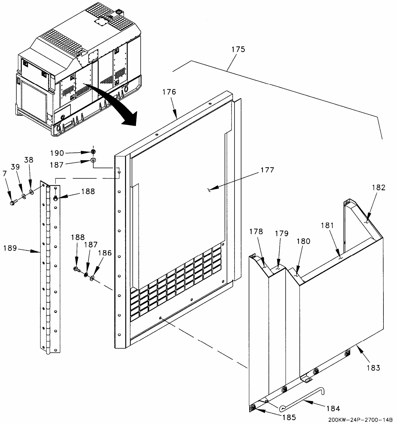
Figure 3. Housing Installation (Sheet 14 of 27).
