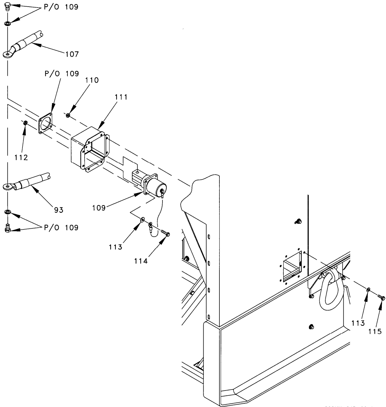
Figure 7. Electrical Components Installation (Sheet 8 of 9).
