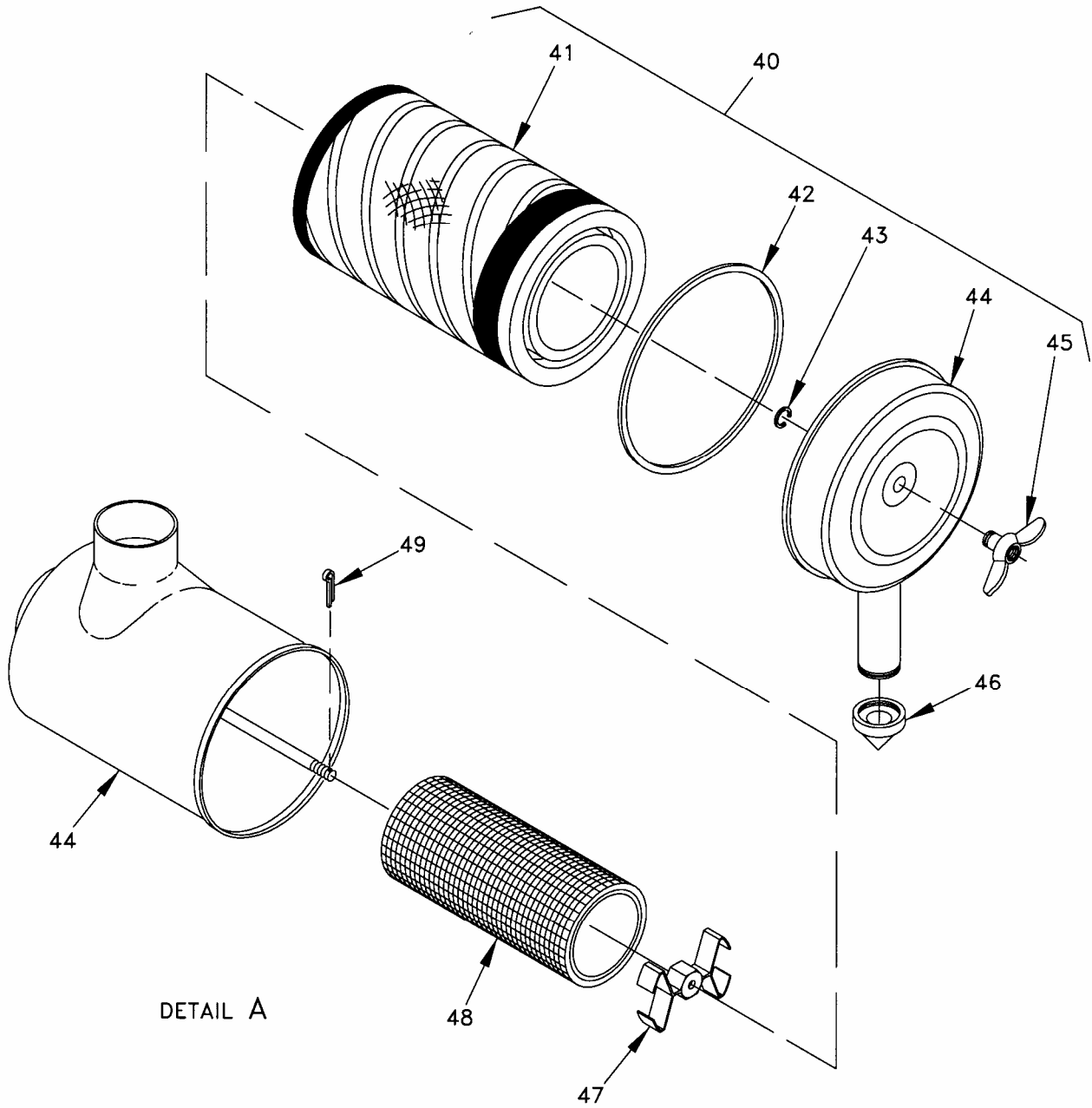
Figure 15. Air Cleaner Installation (Sheet 3 of 3).
