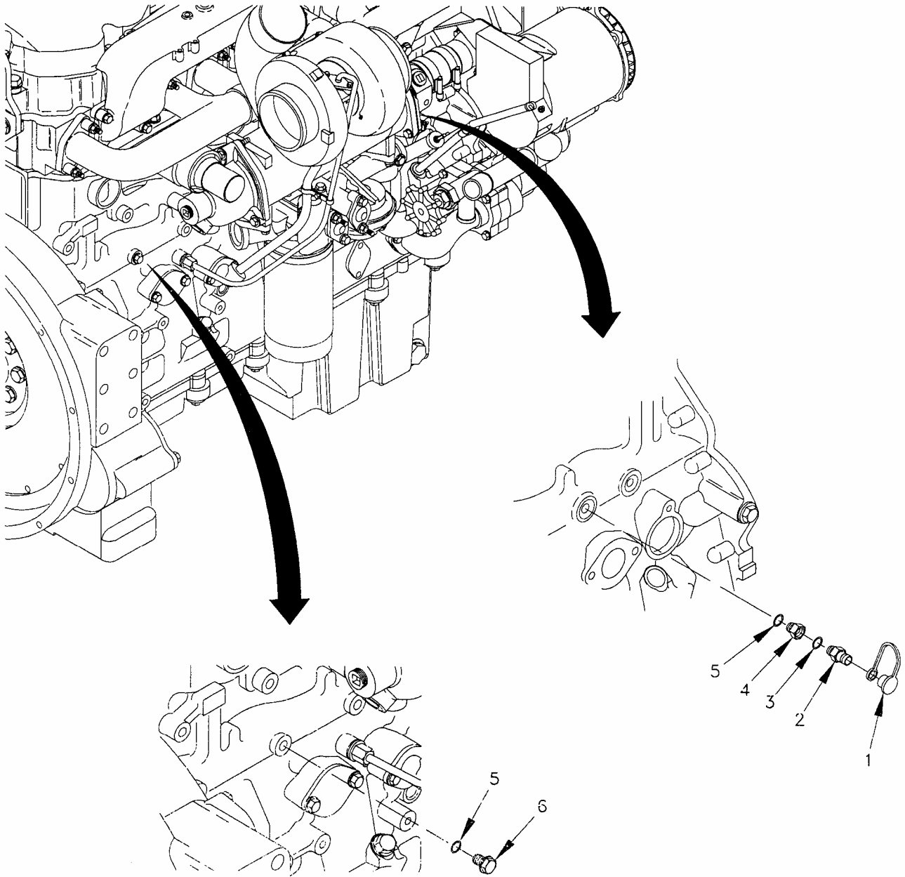
Figure 41. Oil Sampling Group.
