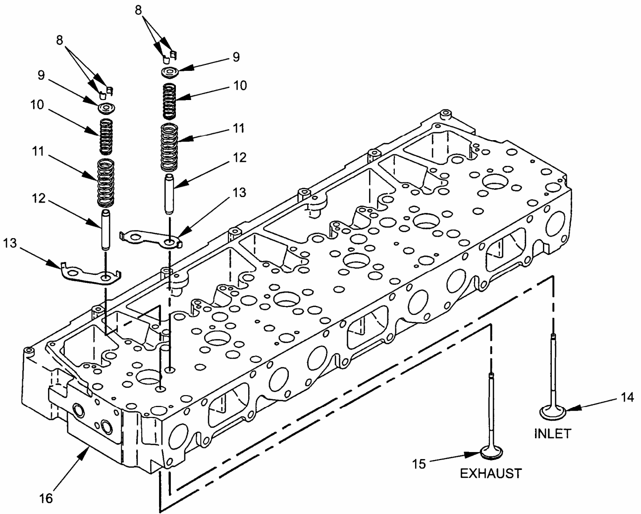
Figure 48. Cylinder Head Group (Sheet 2 of 2).
