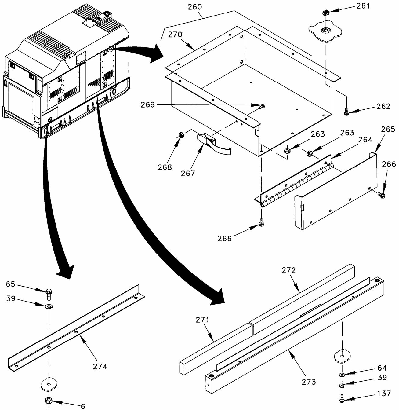
Figure 3. Housing Installation (Sheet 20 of 27).
