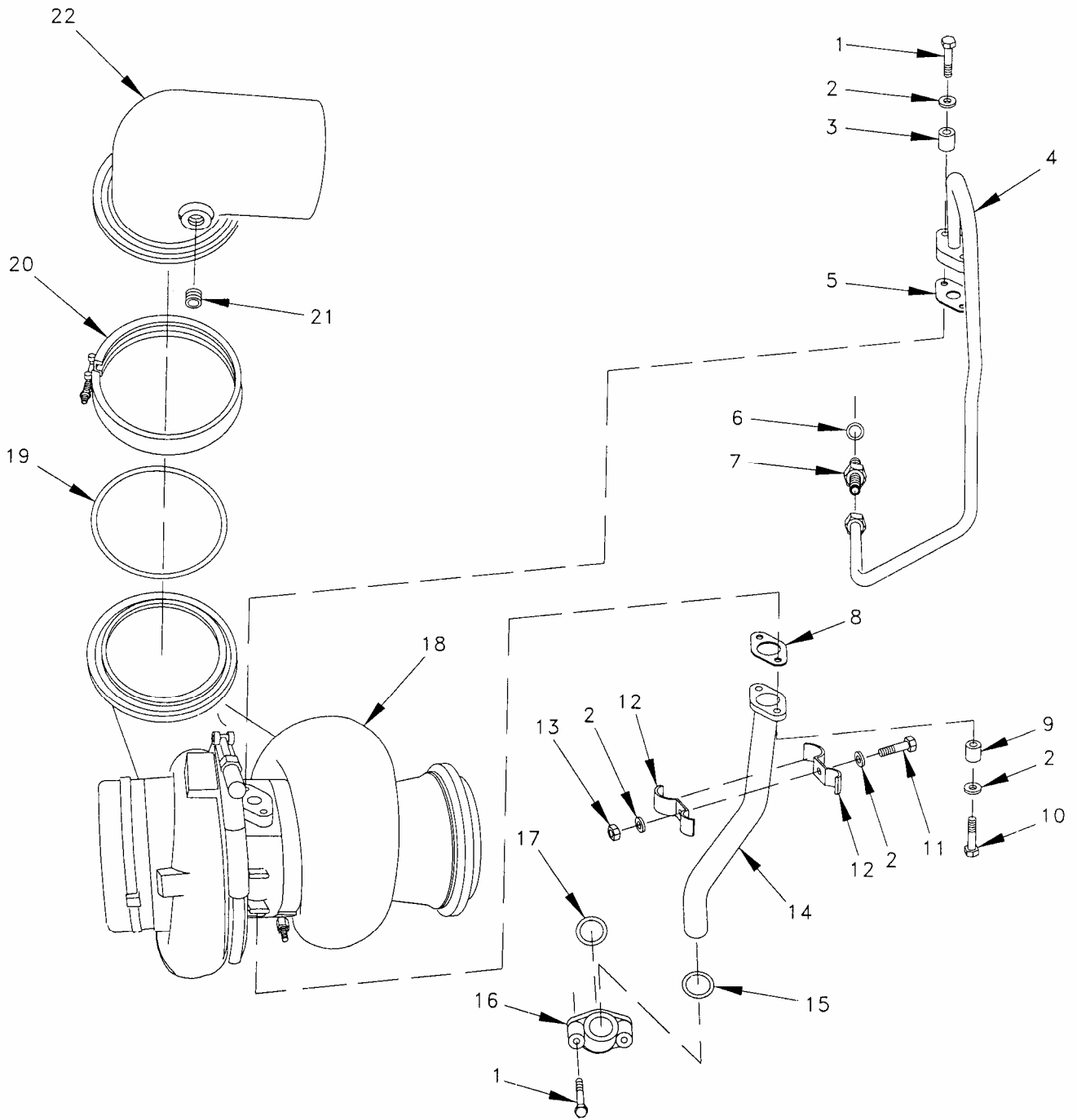
Figure 32. Turbocharger Group.
