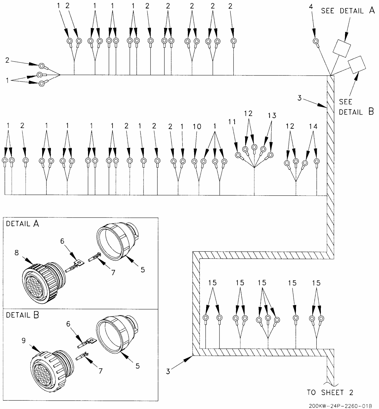
Figure 9. Engine Harness Assembly (Sheet 1 of 3).
