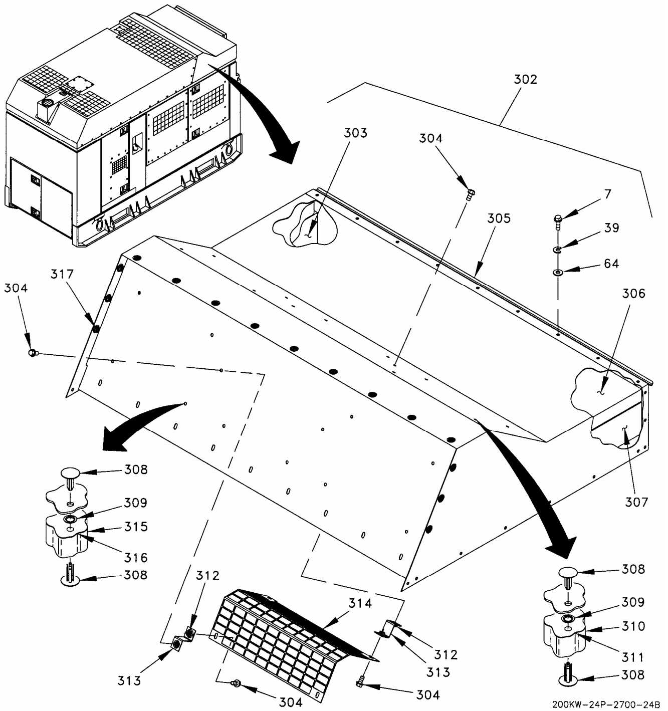
Figure 3. Housing Installation (Sheet 24 of 27).
