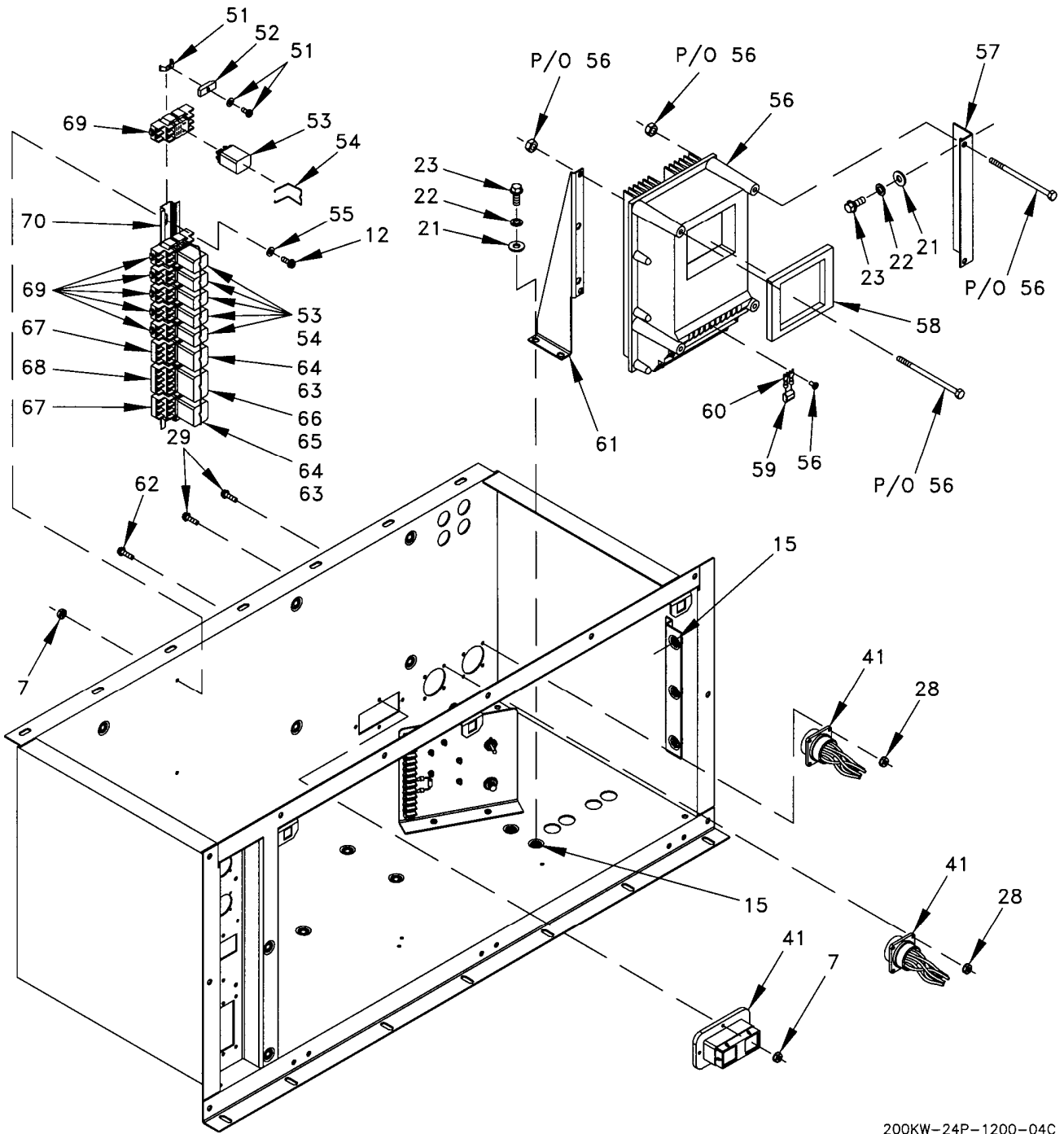
Figure 4. Control Box Assembly (Sheet 4 of 5).
