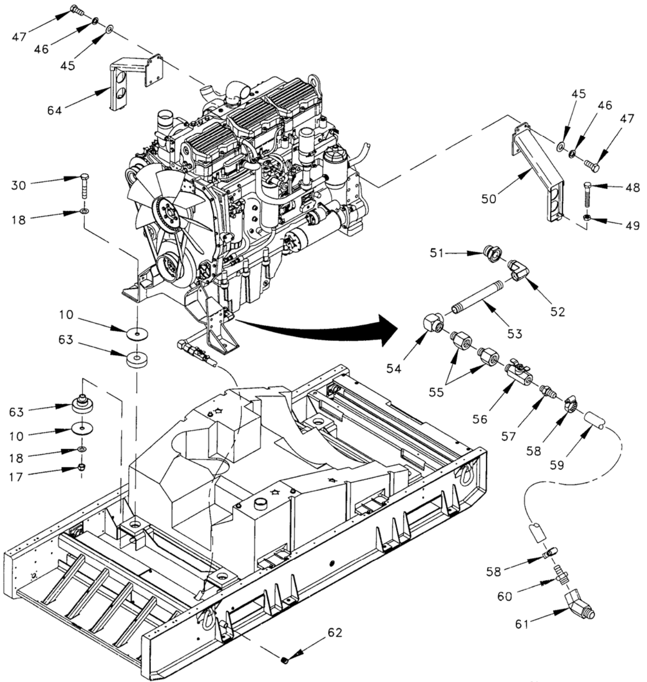
Figure 16. Engine Generator Base Assembly (Sheet 3 of 4).
