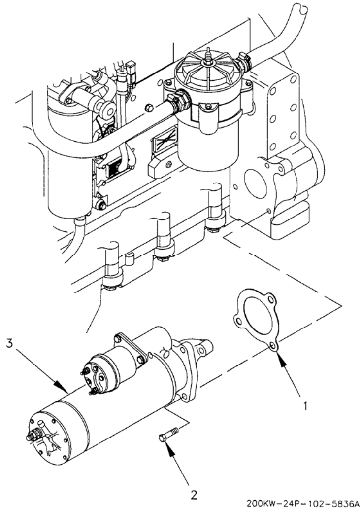
Figure 27. Starter Group.
