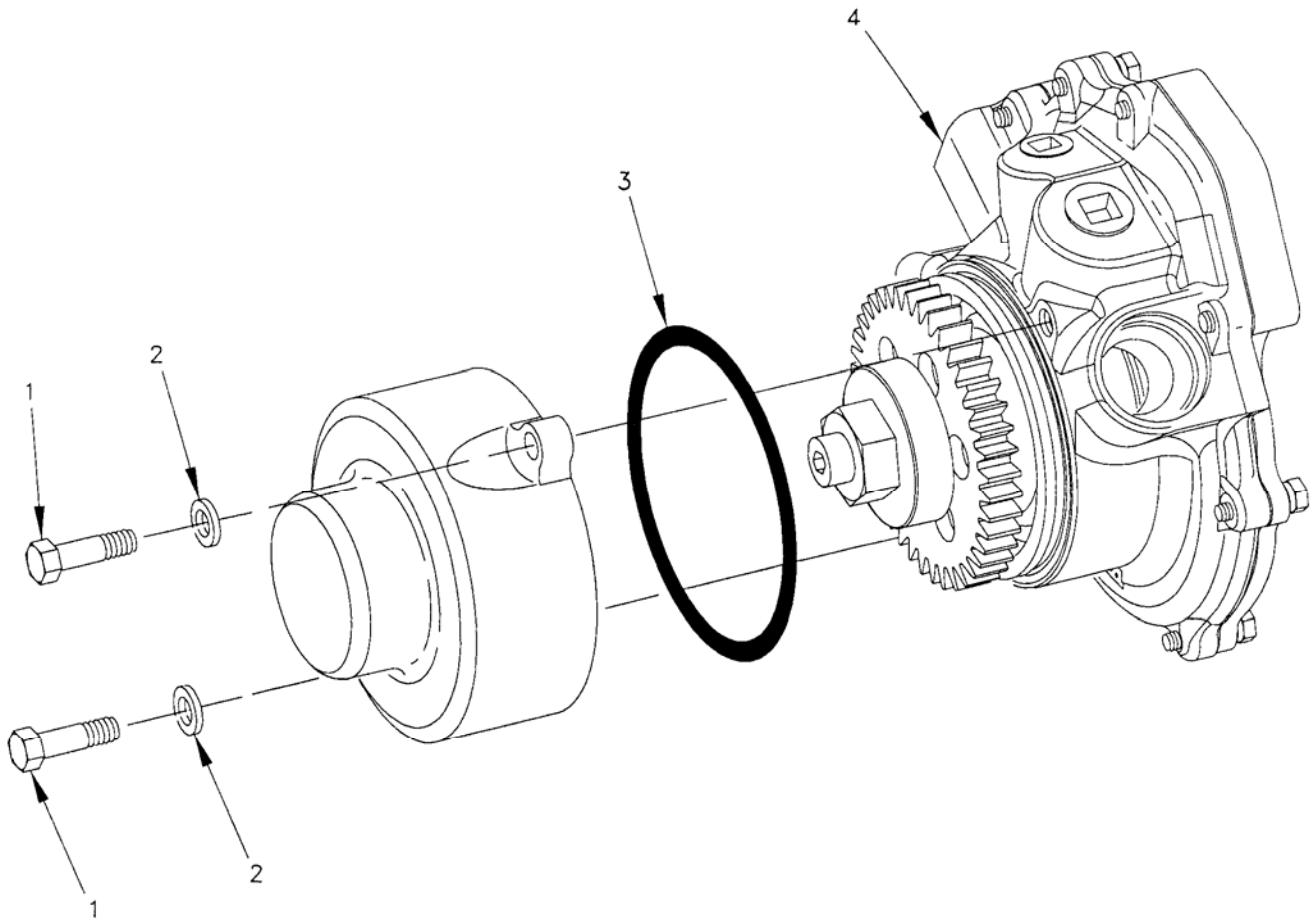
Figure 25. Water Pump Group.
