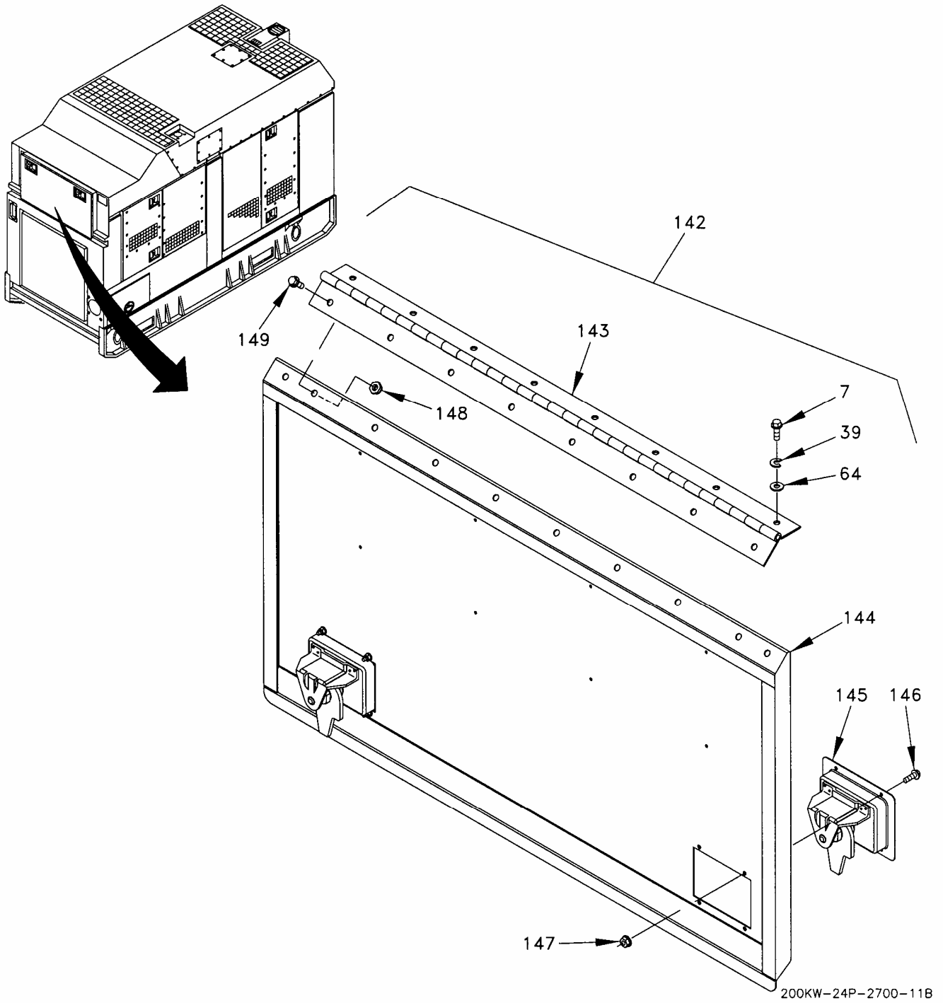
Figure 3. Housing Installation (Sheet 11 of 27).
