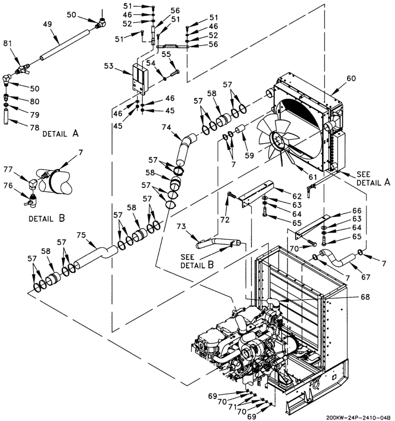
Figure 13. Cooling System Installation (Sheet 4 of 6).
