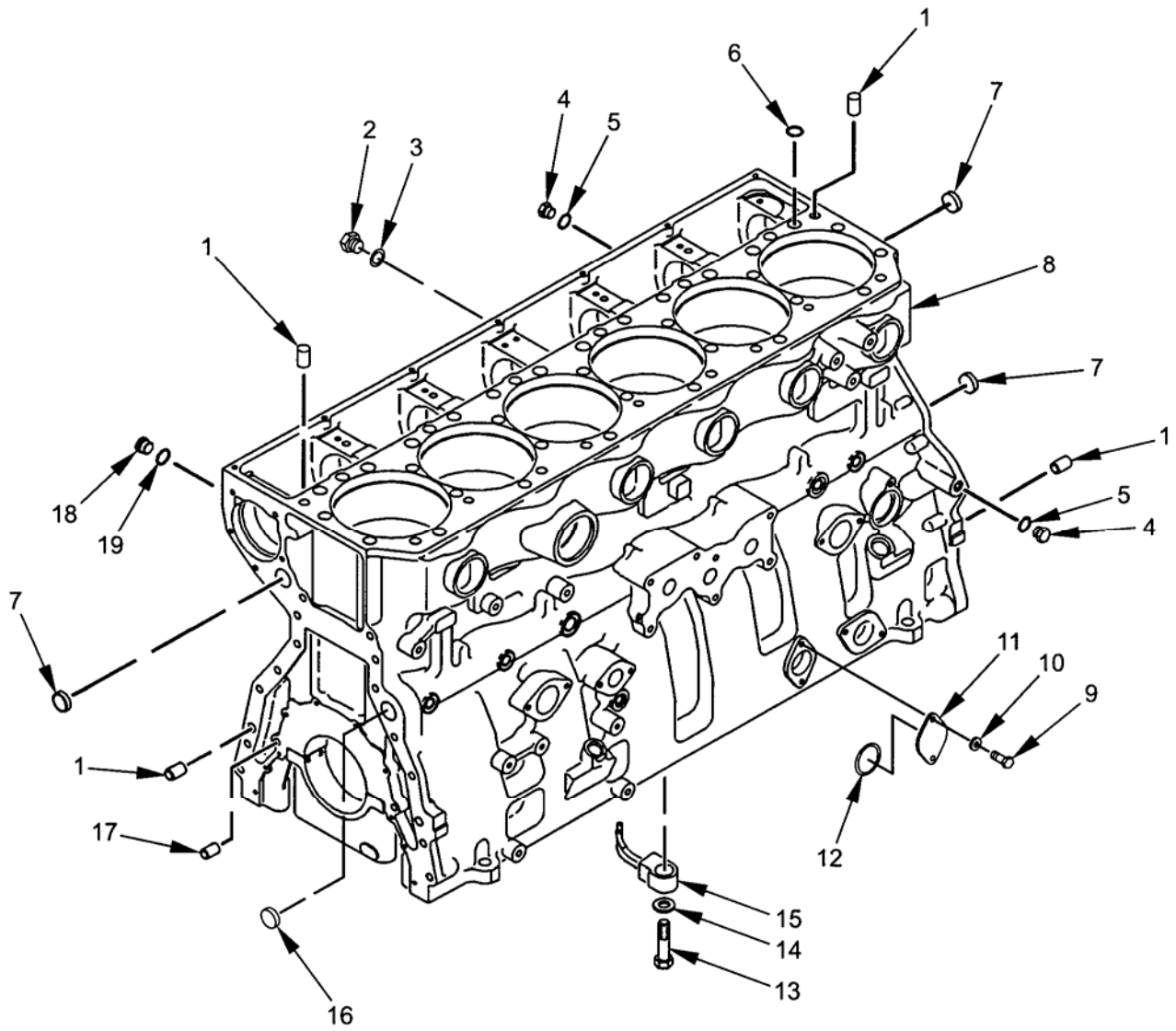
Figure 59. Block Group.
