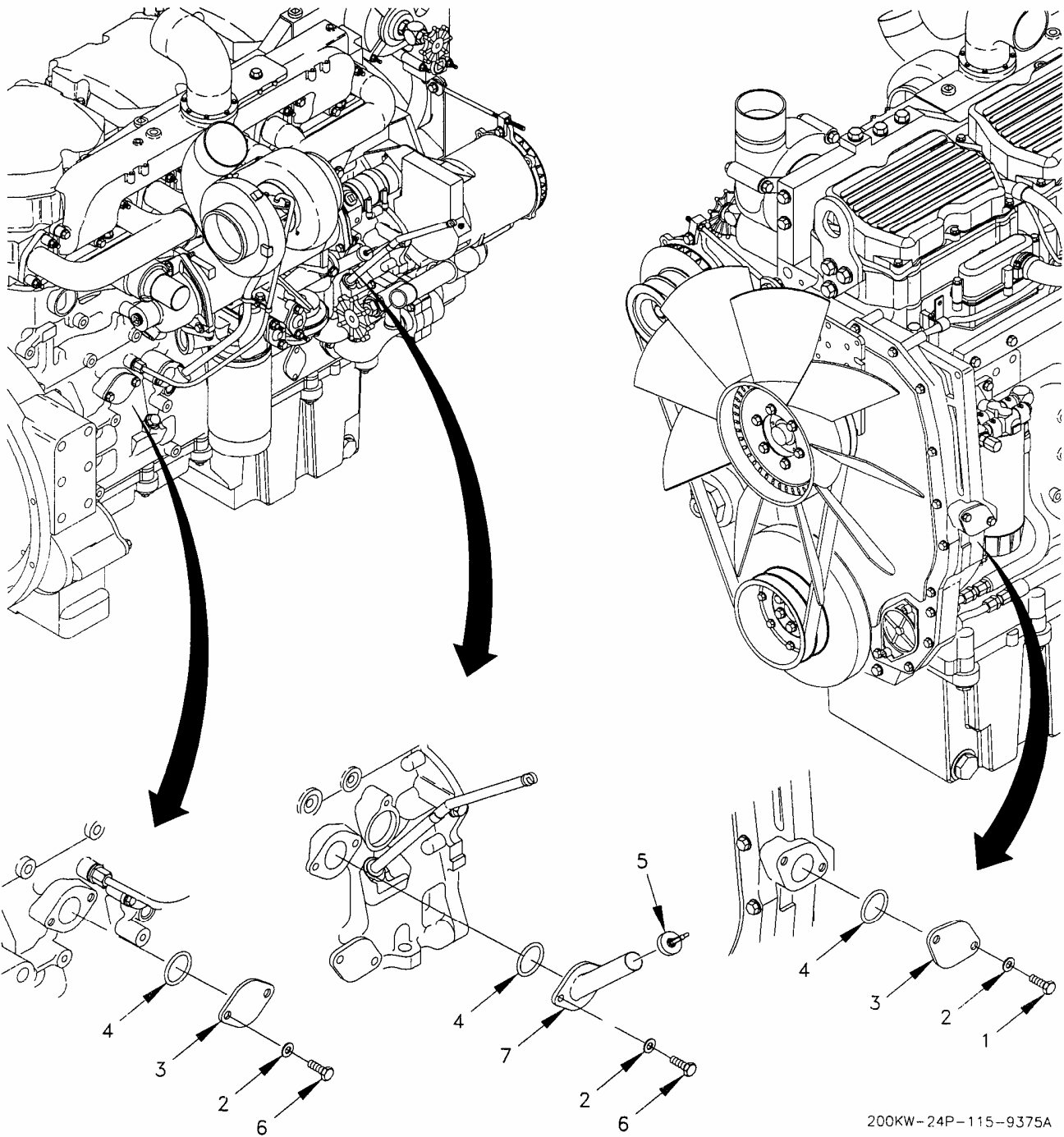
Figure 39. Oil Filler Group.
