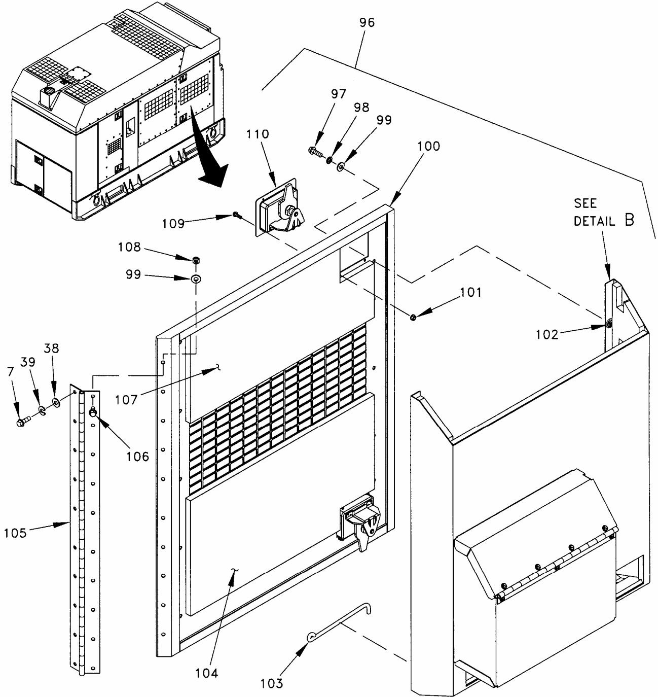
Figure 3. Housing Installation (Sheet 7 of 27).
