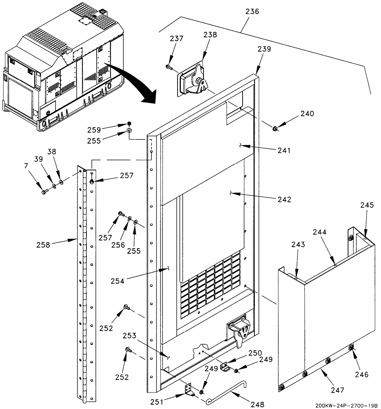
Figure 3. Housing Installation (Sheet 19 of 27).
