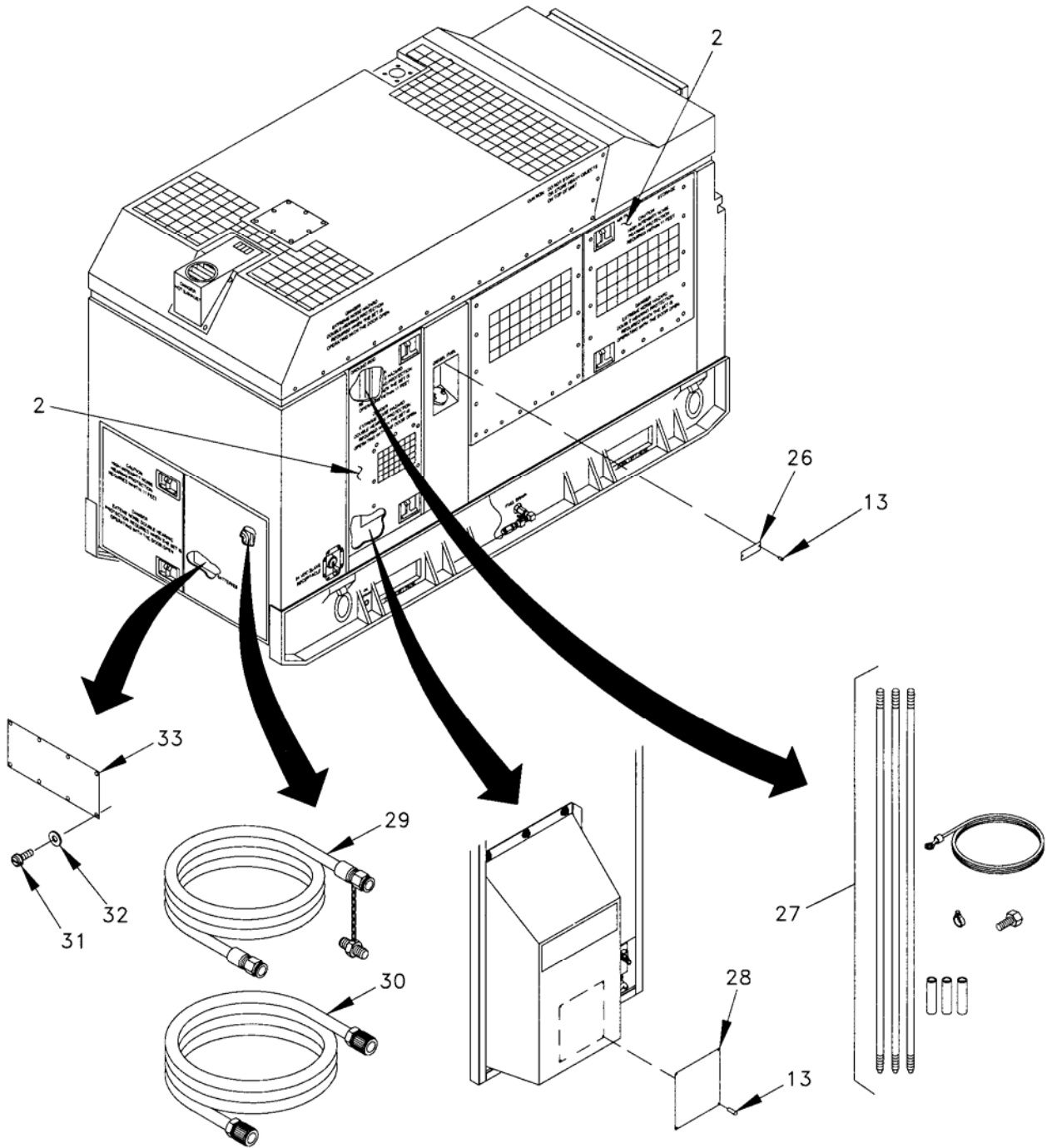
Figure 1. Generator Set, Tactical Quiet, 200 kW, 50/60 Hz (Sheet 2 of 2).
